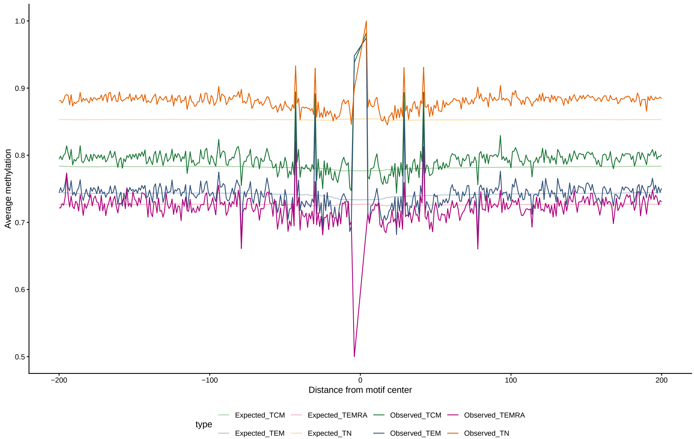
Expected vs observed footprints for MEIS1(var.2)
