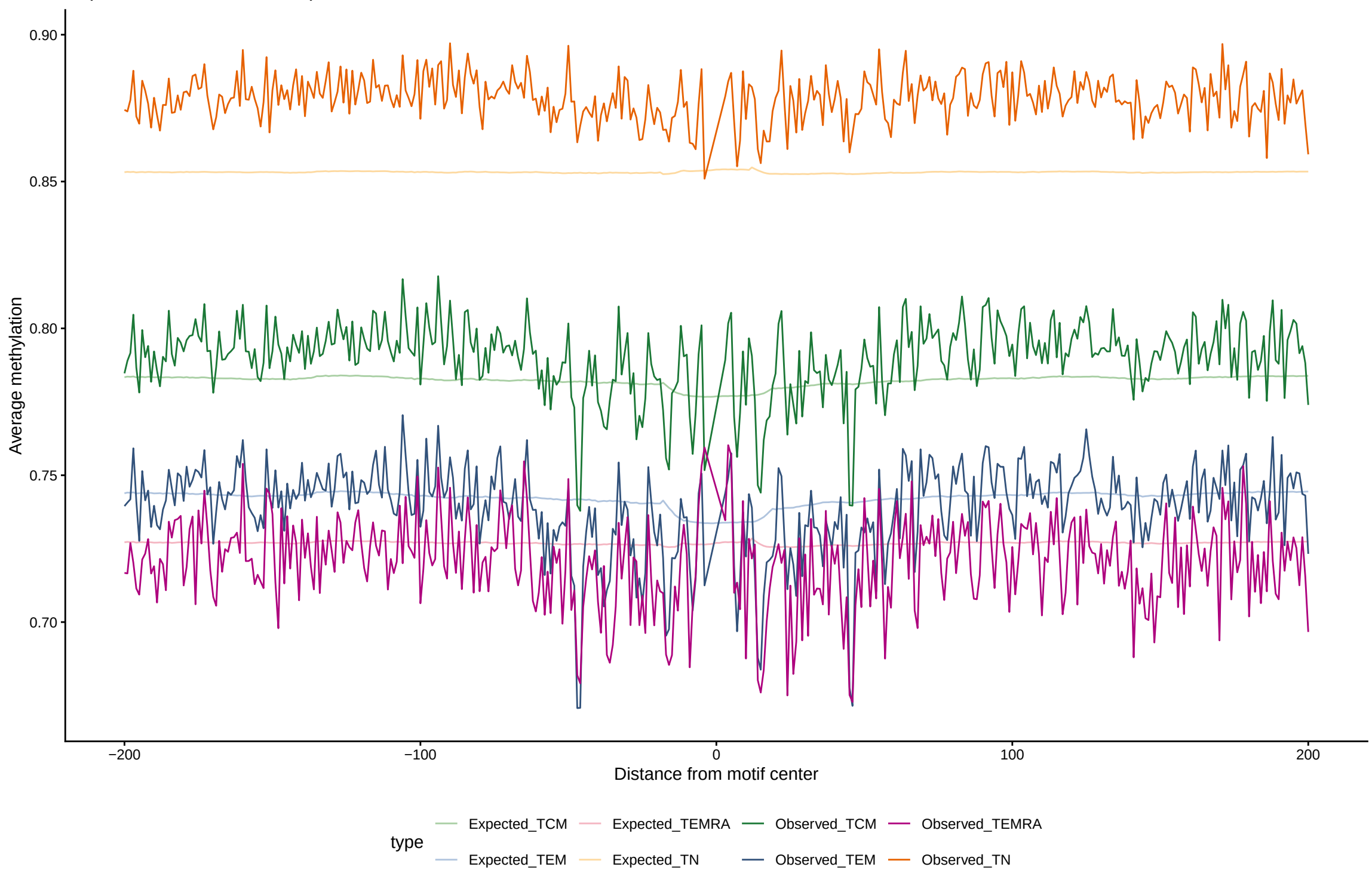
Expected vs observed footprints for MEOX1
