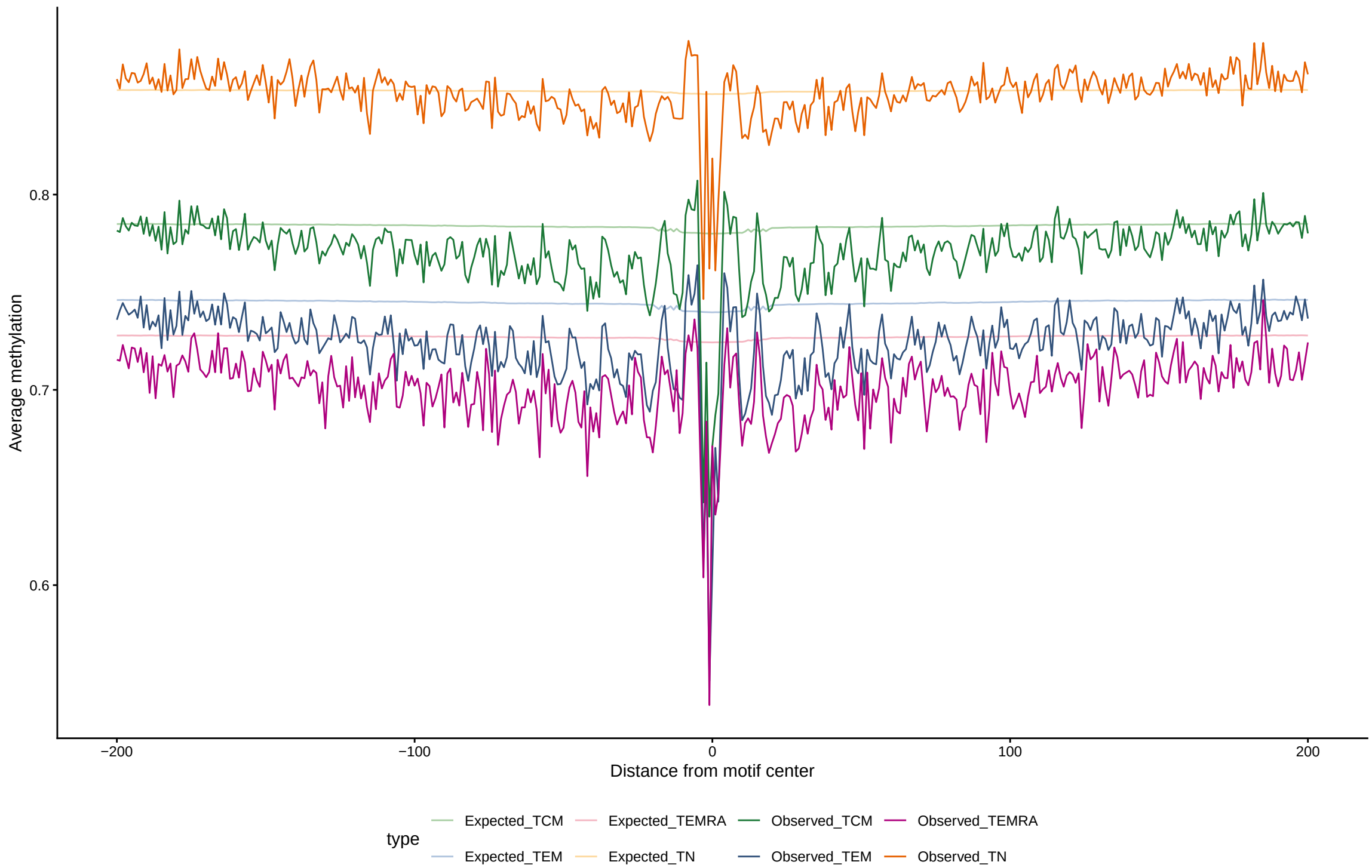
Expected vs observed footprints for MYF6
