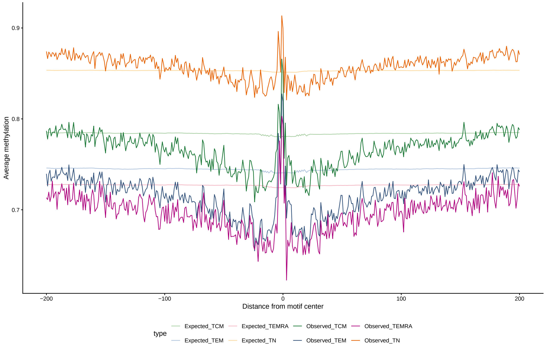
Expected vs observed footprints for NFE2L1
