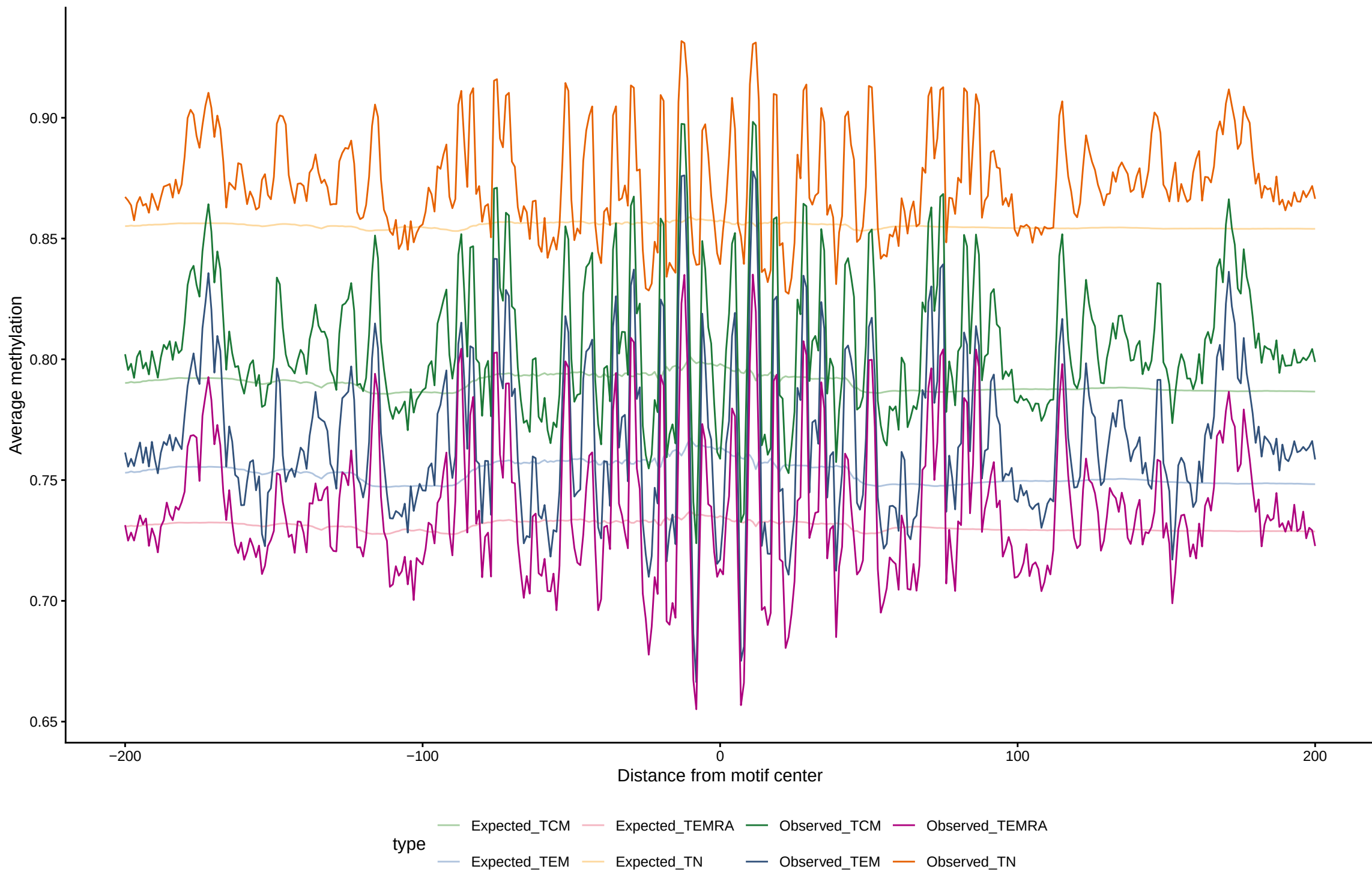
Expected vs observed footprints for NFIC::TLX1
