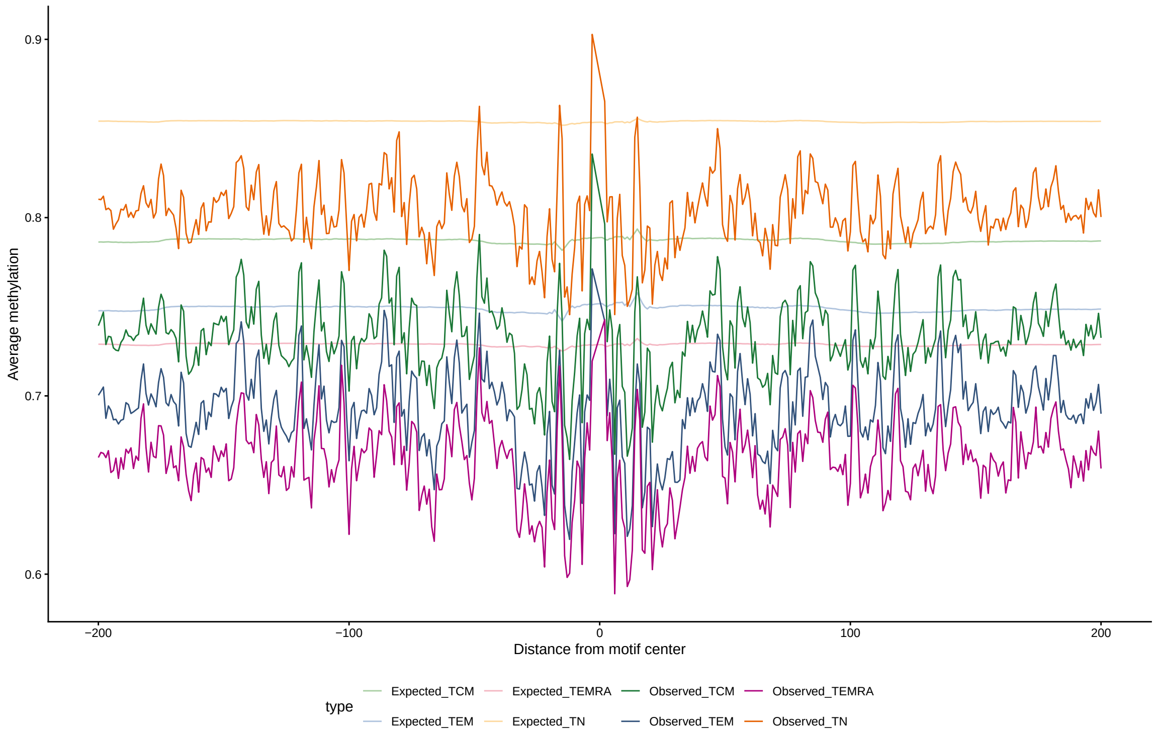
Expected vs observed footprints for NFYB
