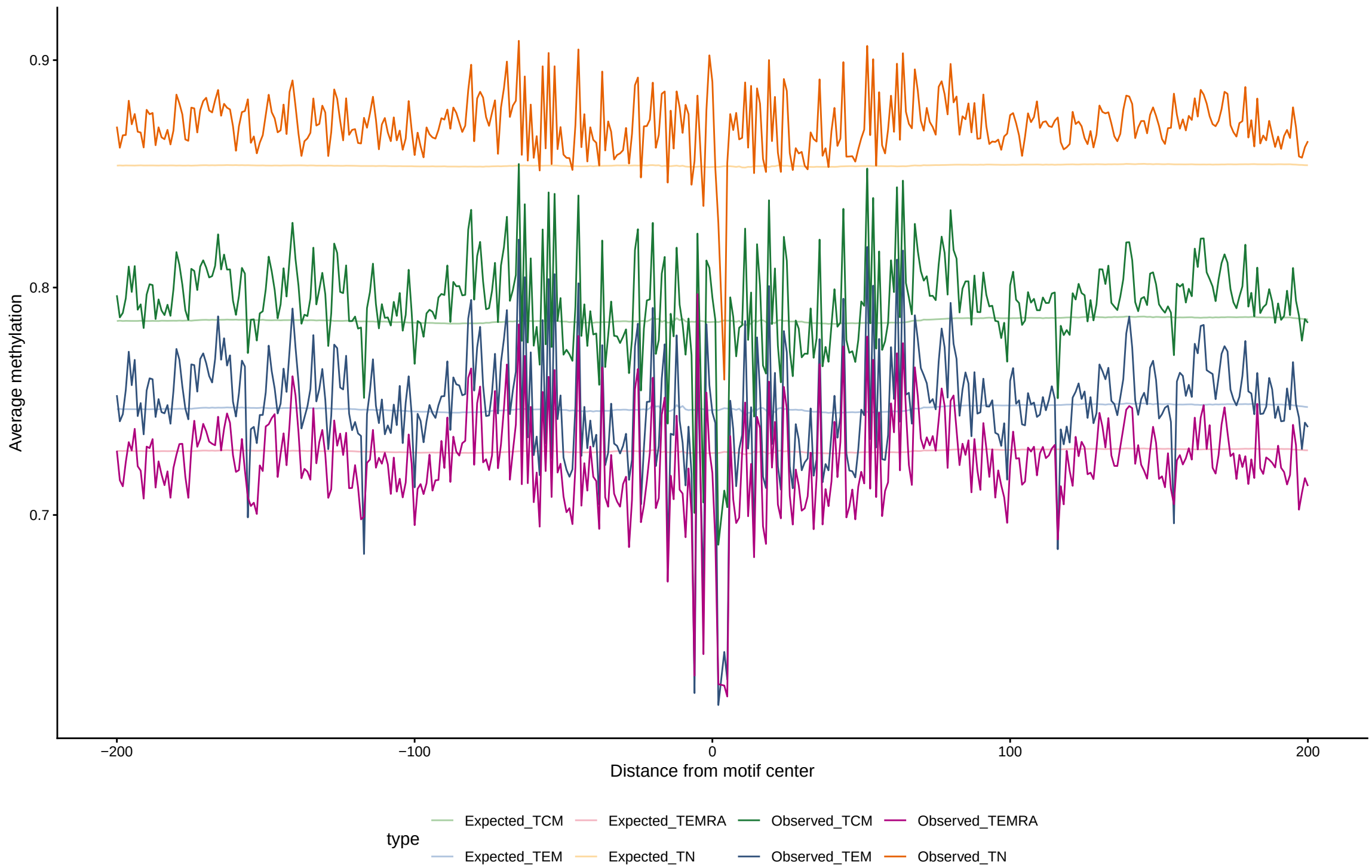
Expected vs observed footprints for NR1D2
