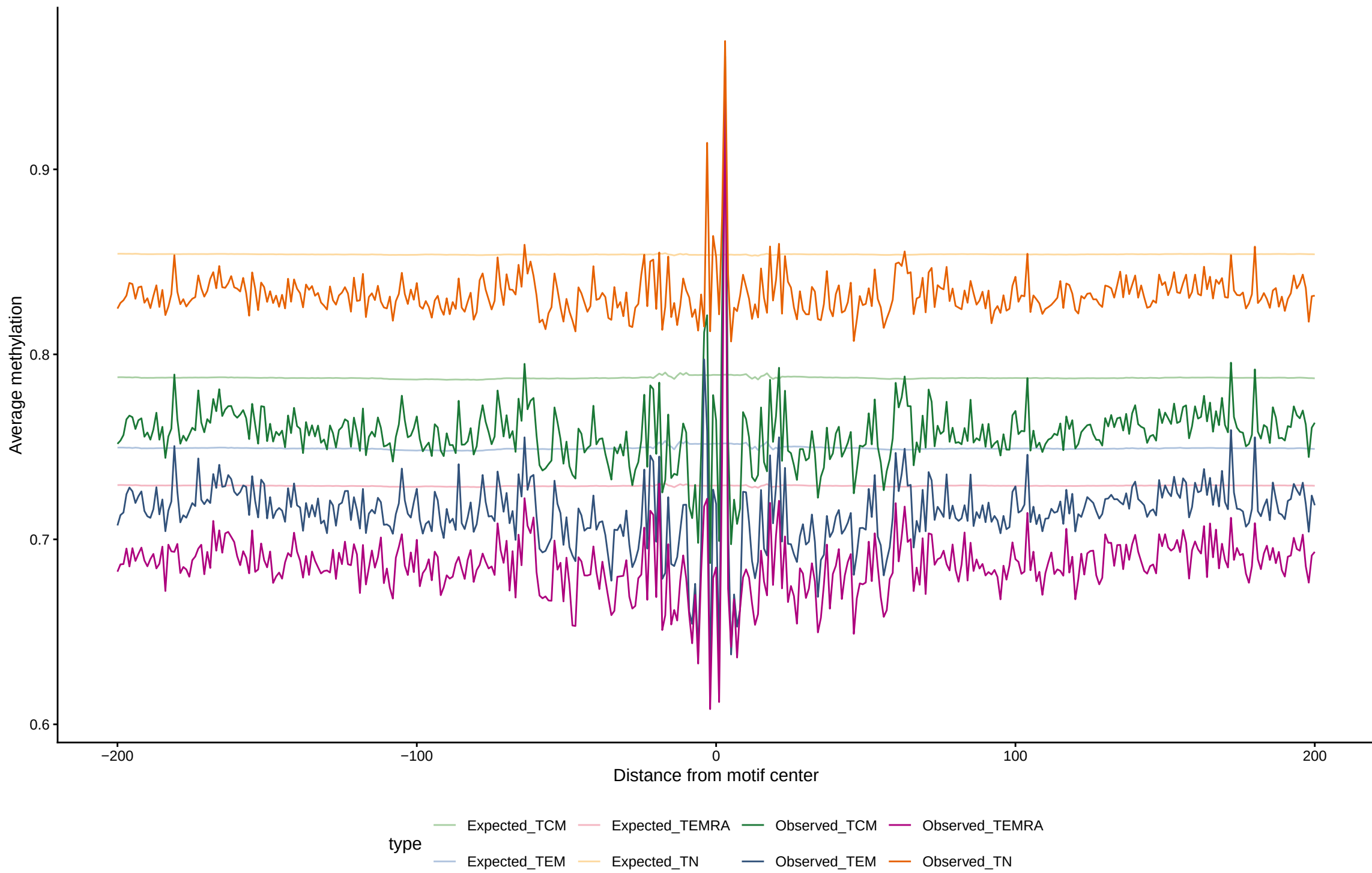
Expected vs observed footprints for NR2F1(var.2)
