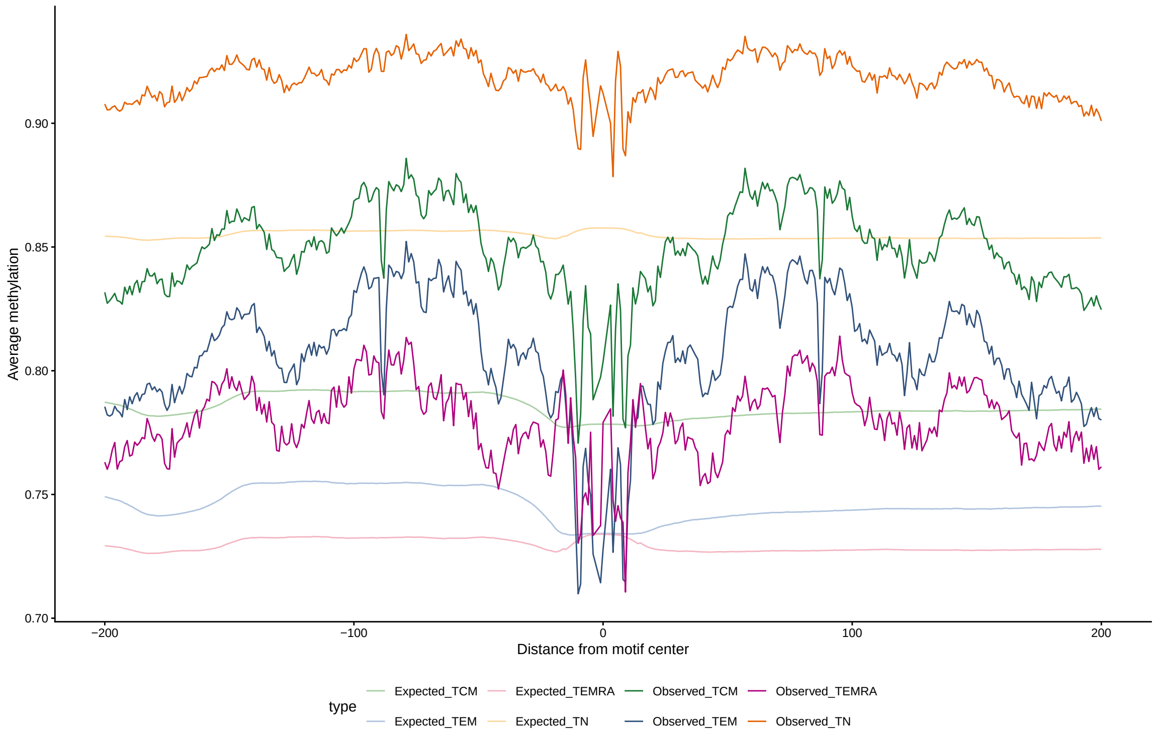
Expected vs observed footprints for ONECUT1
