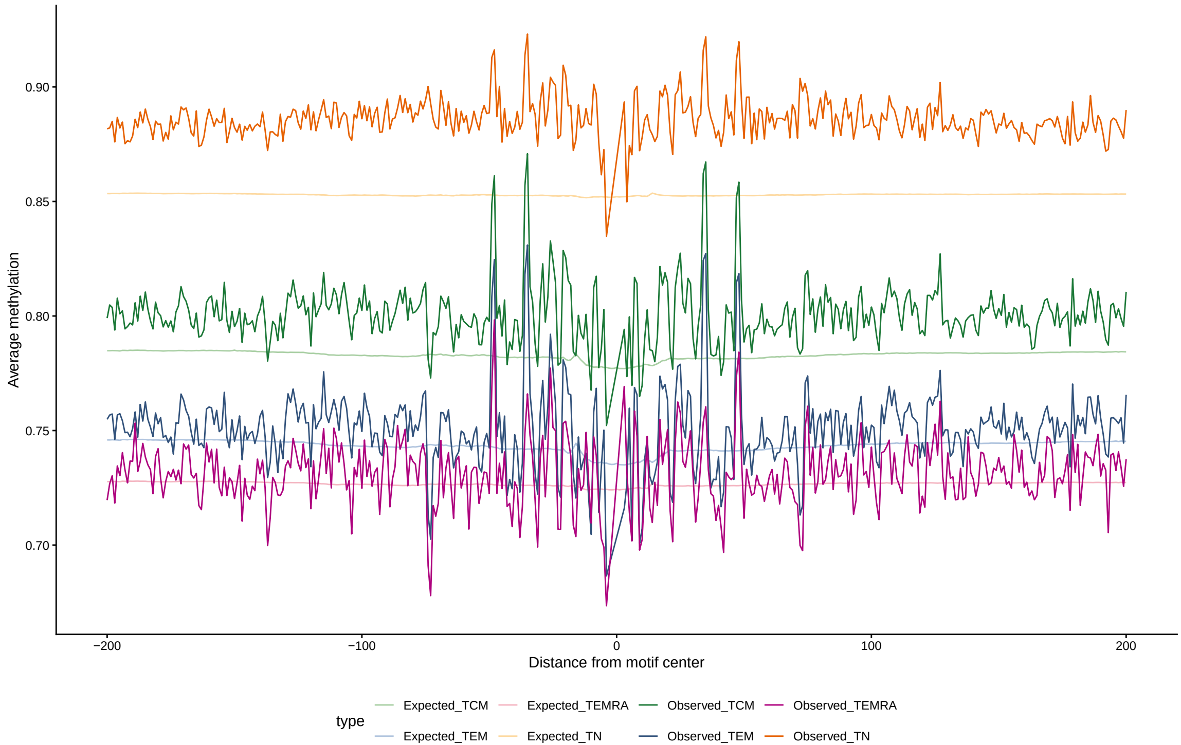
Expected vs observed footprints for OTX2
