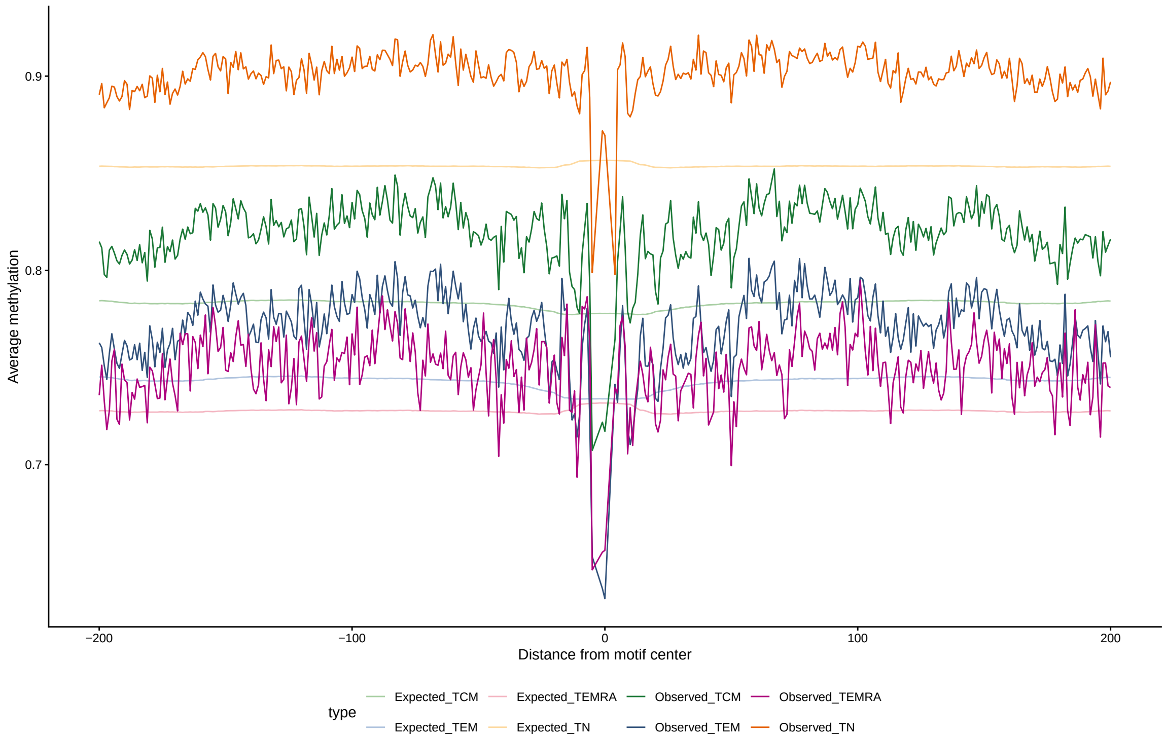
Expected vs observed footprints for PAX7
