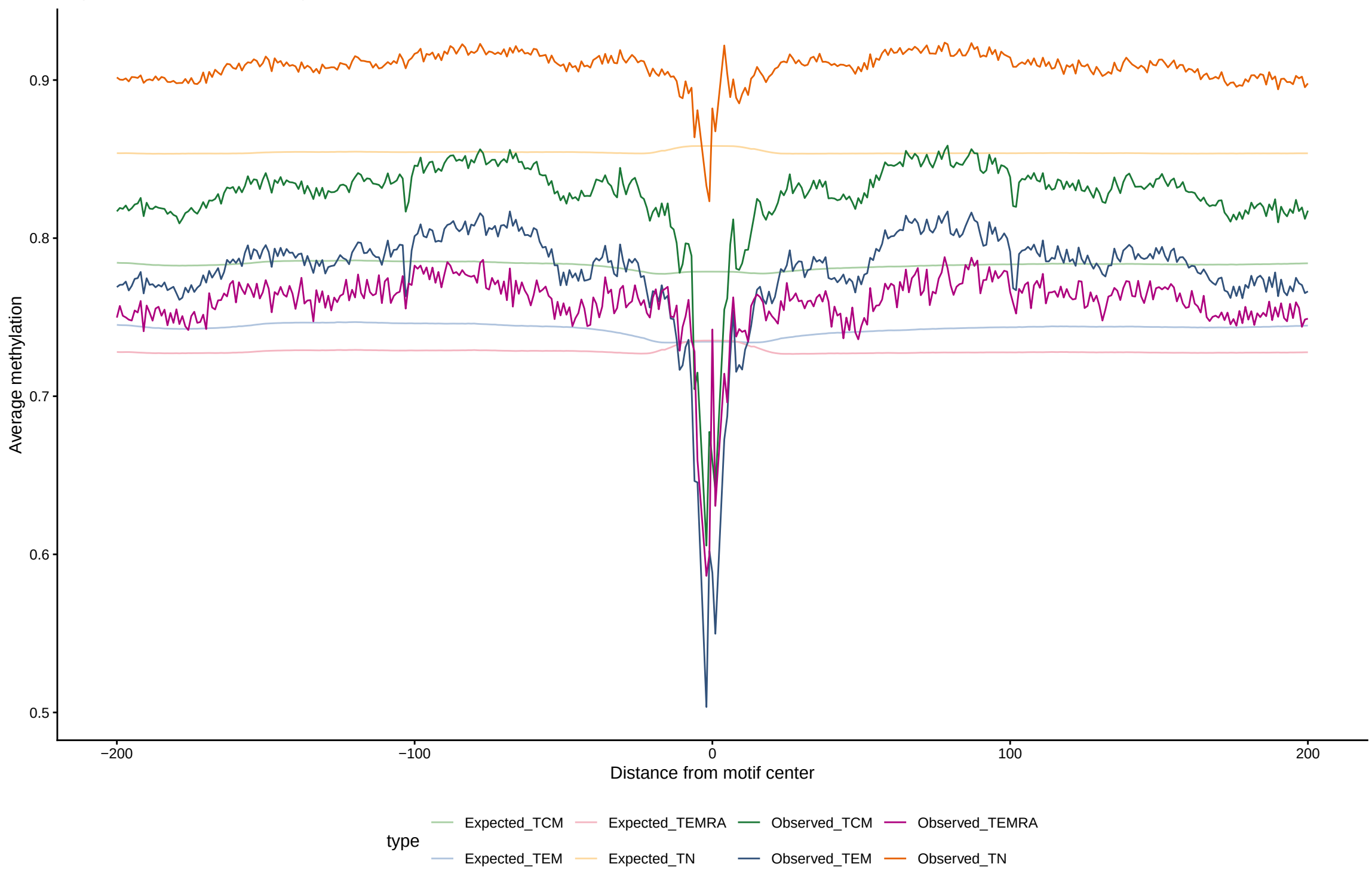
Expected vs observed footprints for PHOX2B
