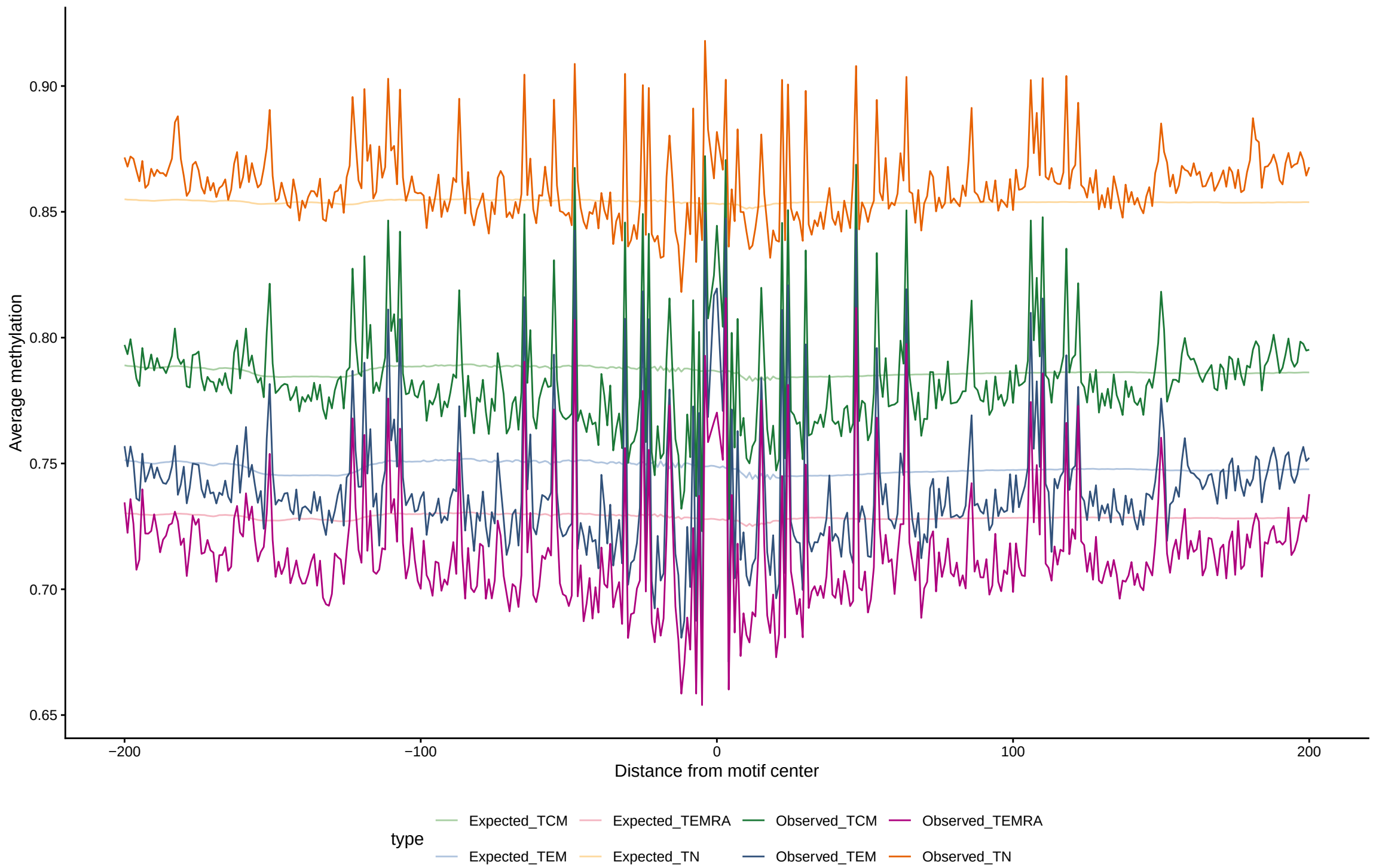
Expected vs observed footprints for PKNOX1
