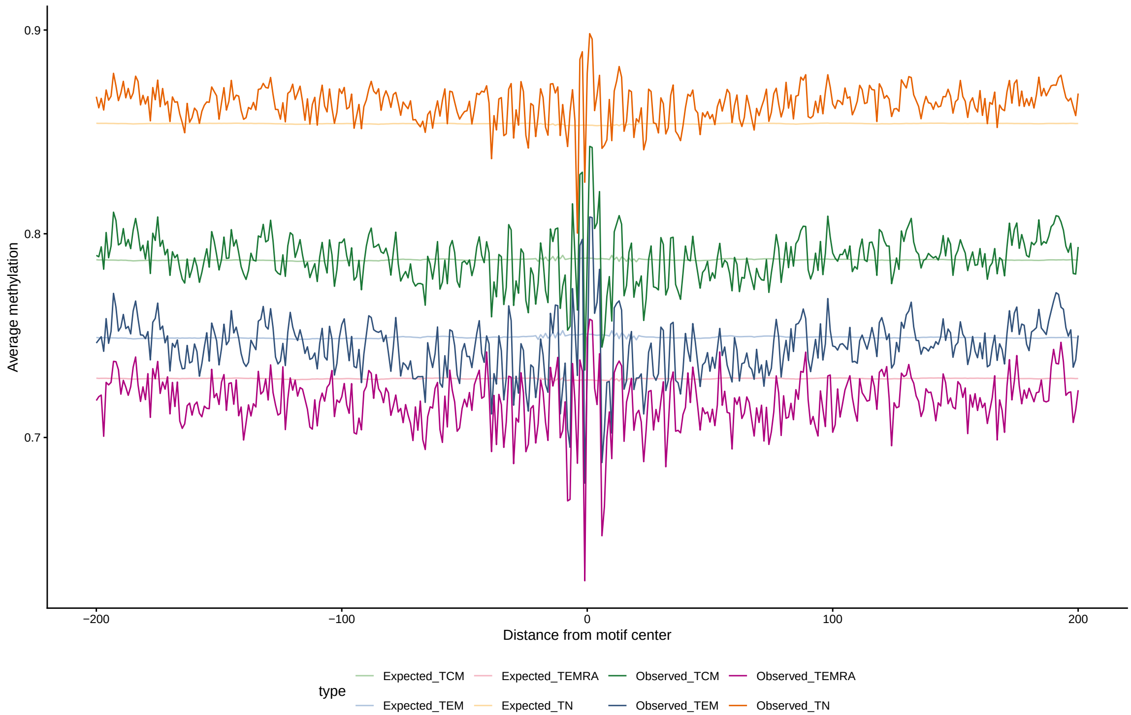
Expected vs observed footprints for PKNOX2
