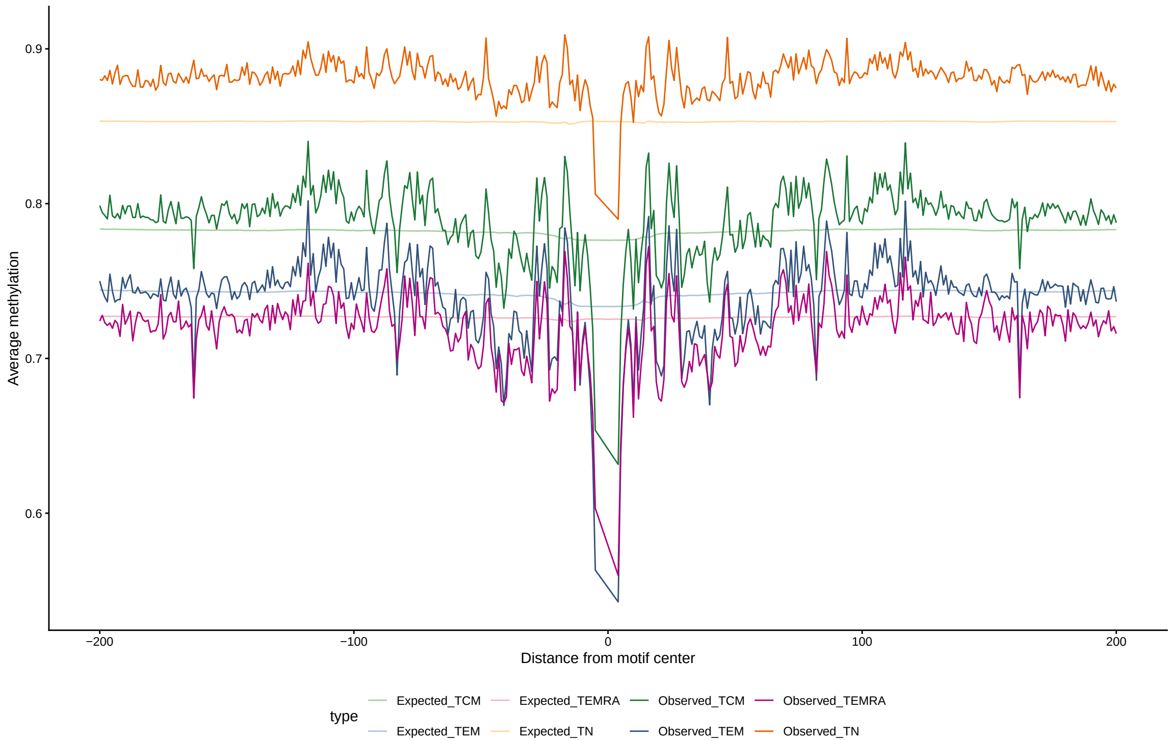
Expected vs observed footprints for POU5F1
