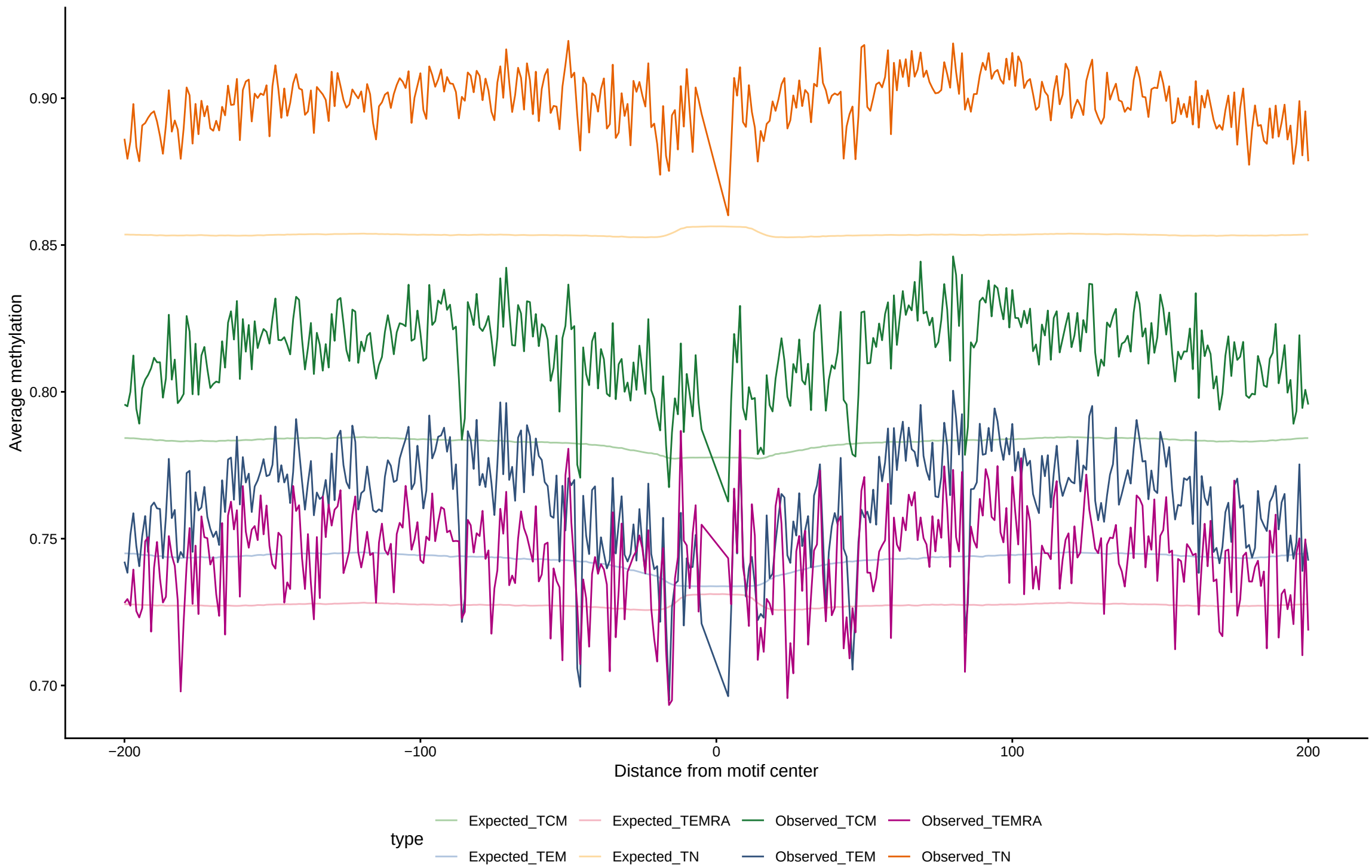
Expected vs observed footprints for POU6F1
