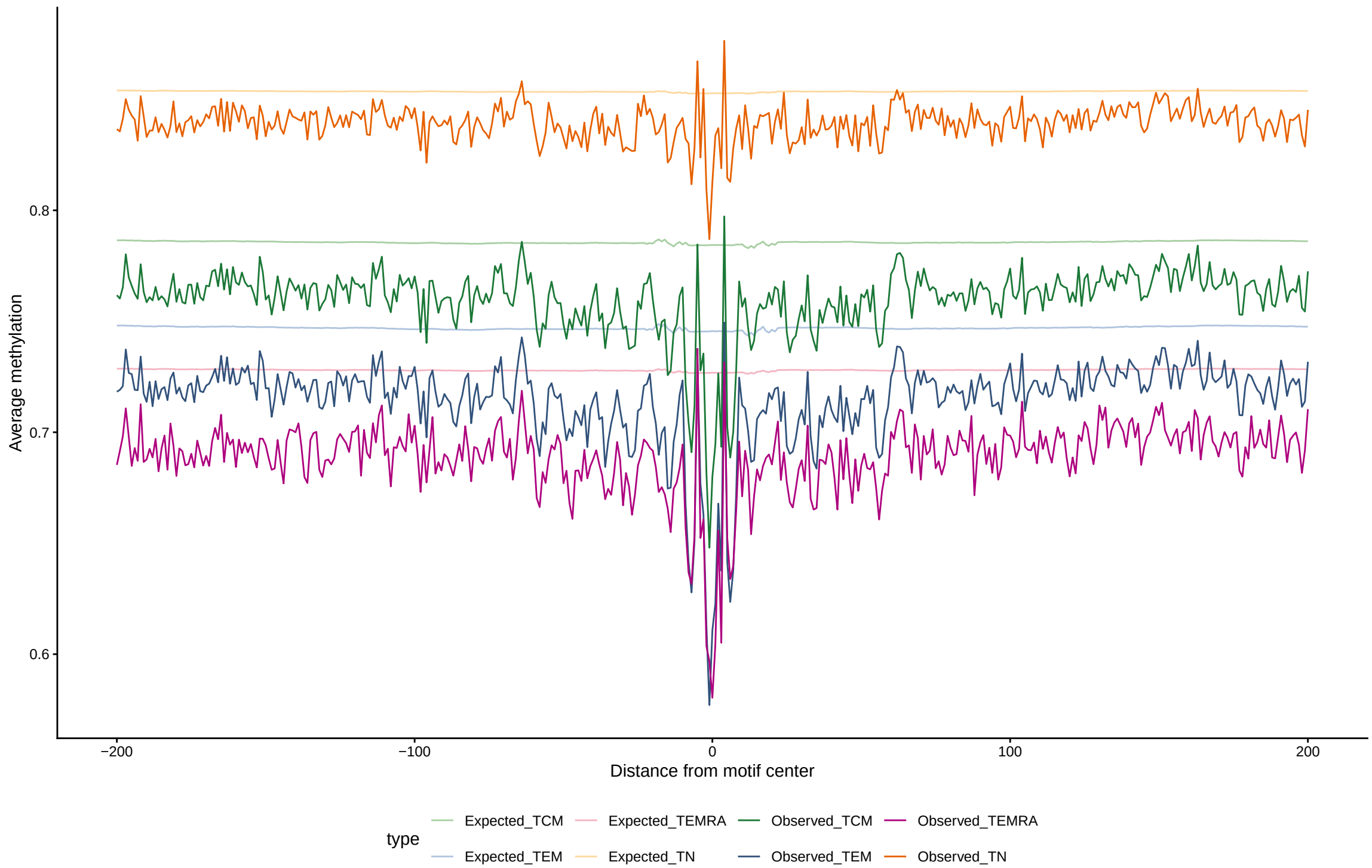
Expected vs observed footprints for PPARD
