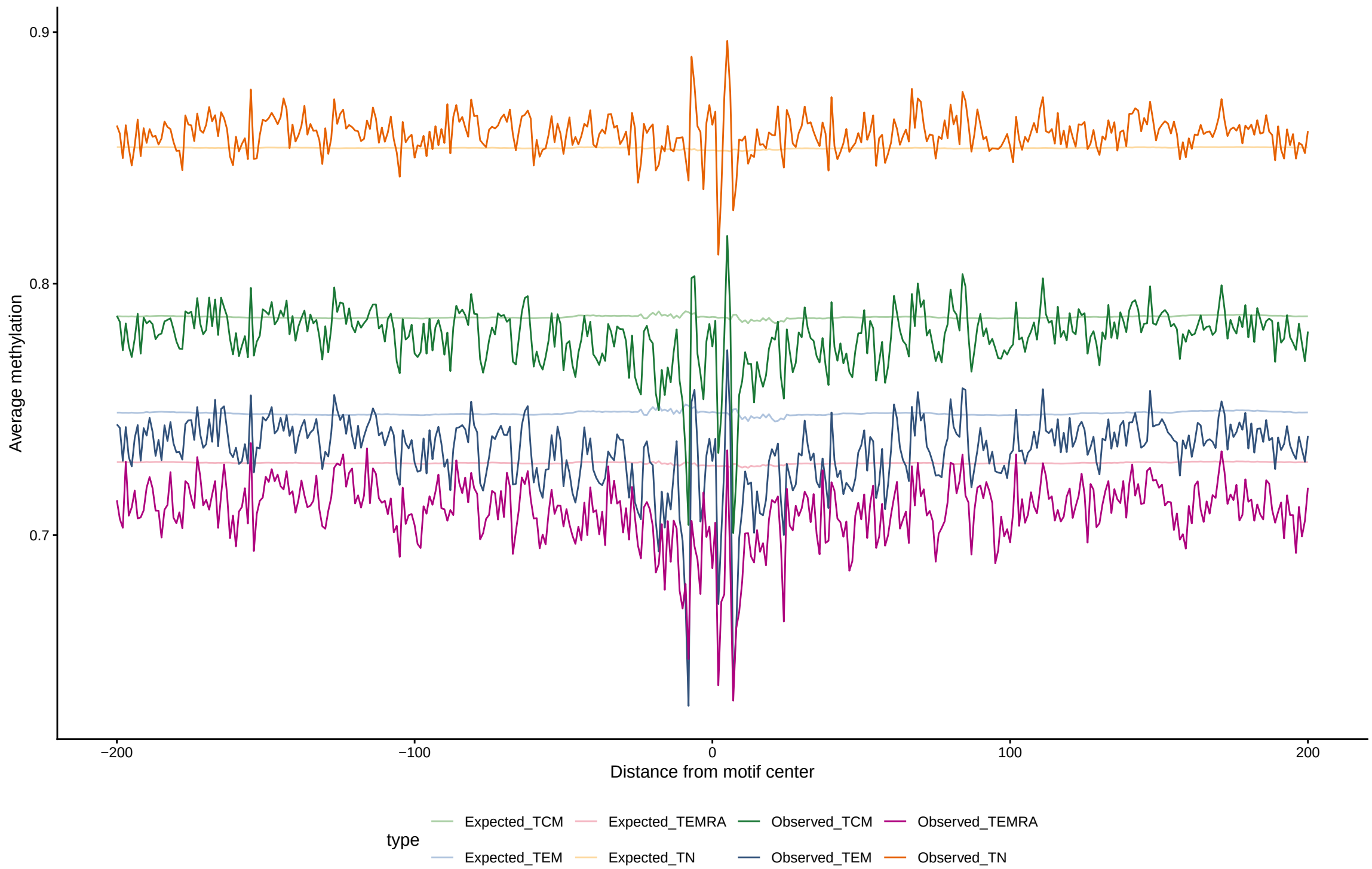
Expected vs observed footprints for PPARG
