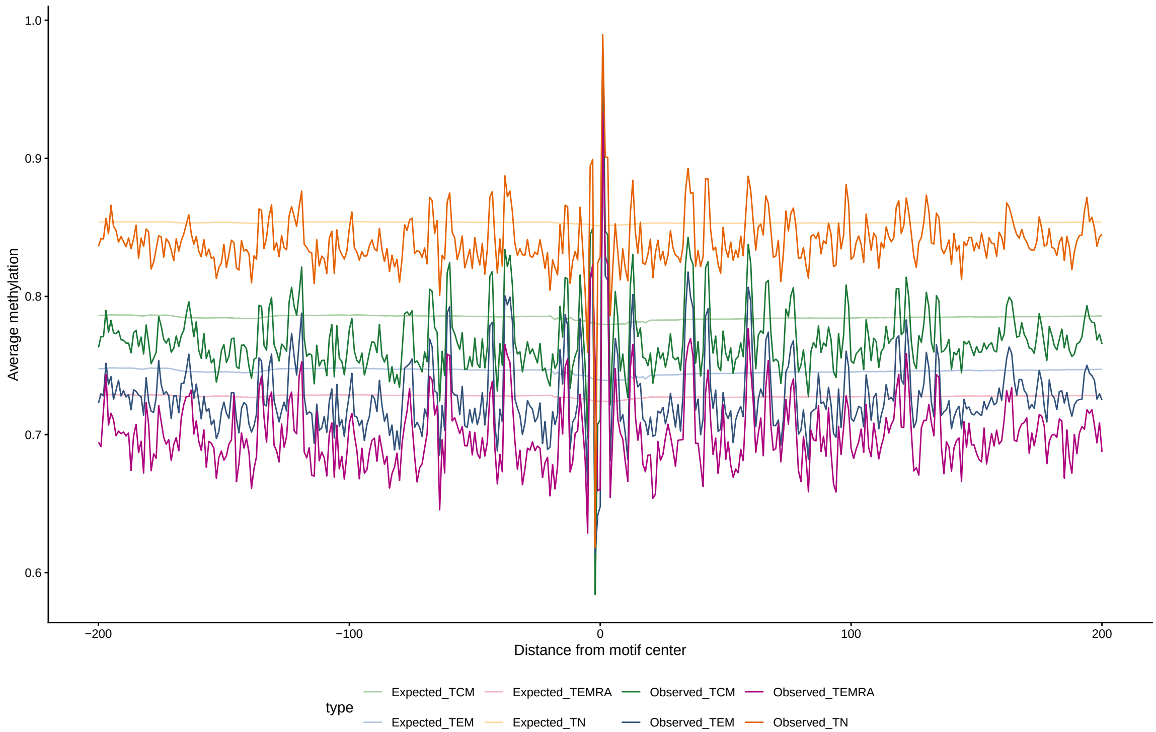
Expected vs observed footprints for PROX1
