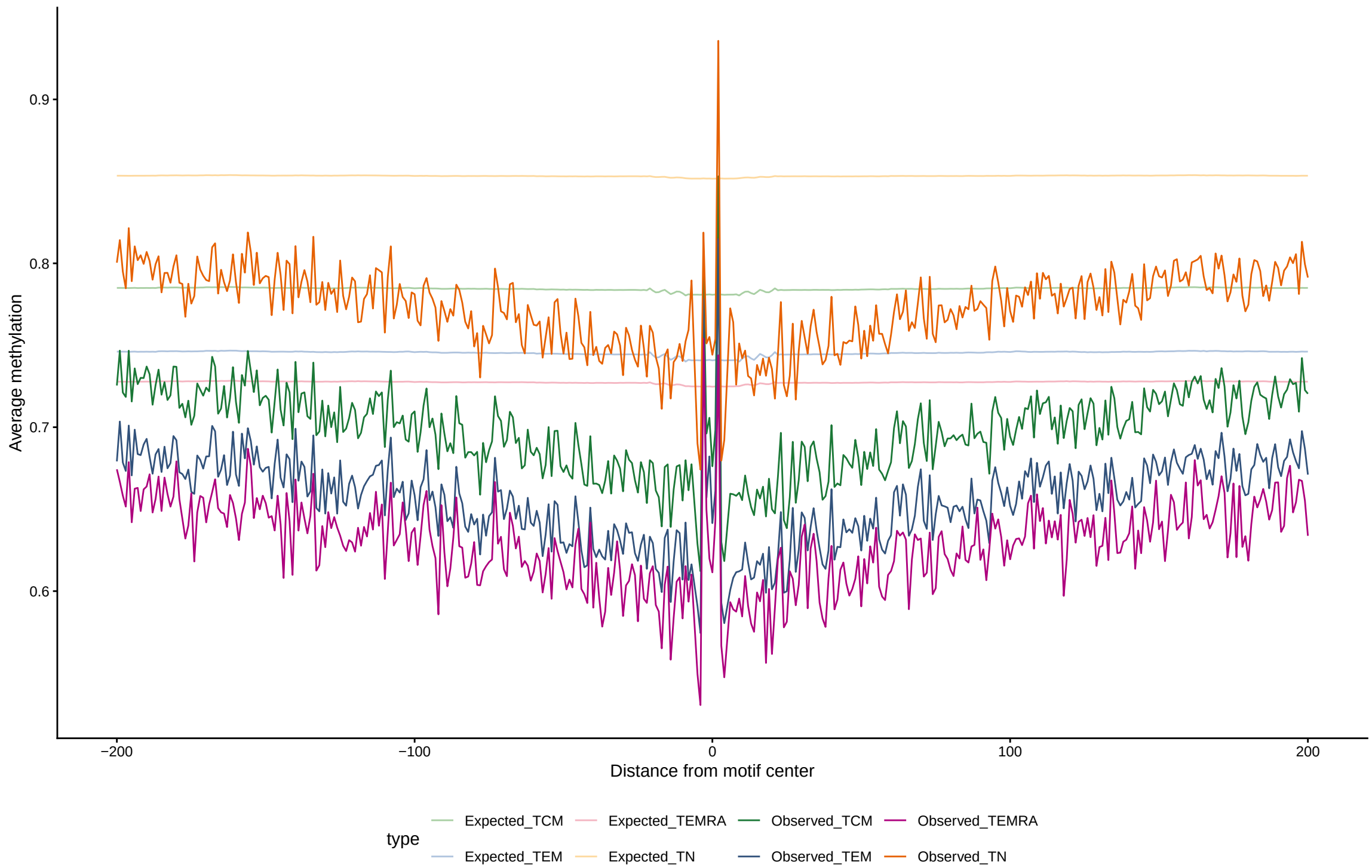
Expected vs observed footprints for RFX2
