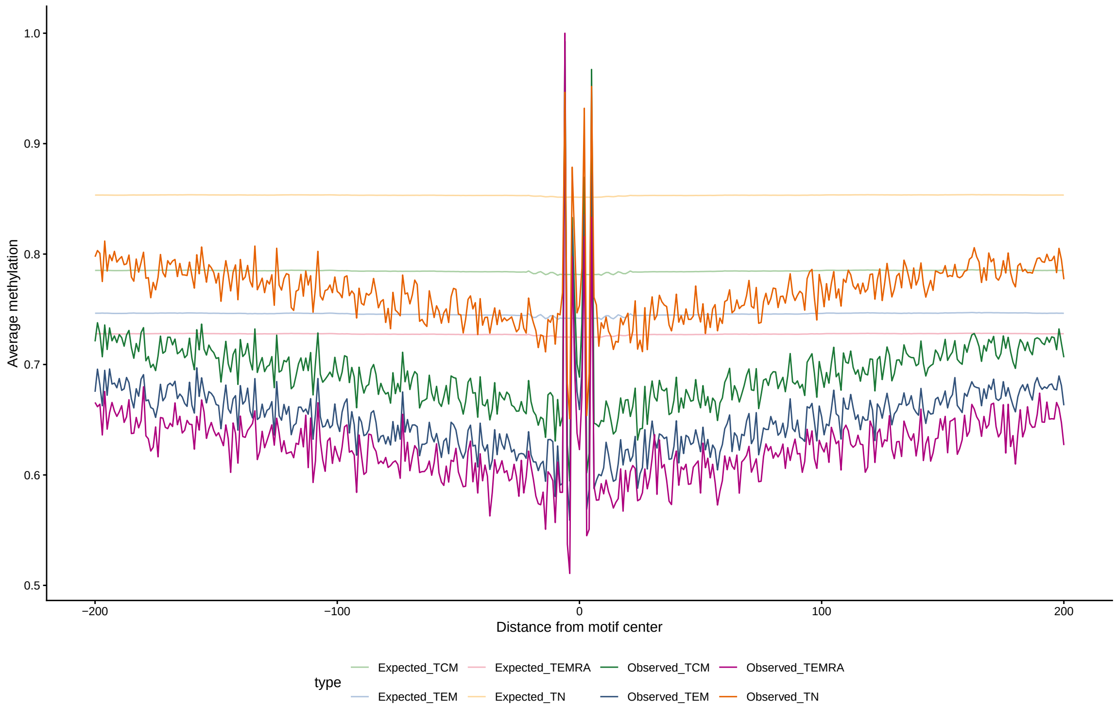
Expected vs observed footprints for RFX5
