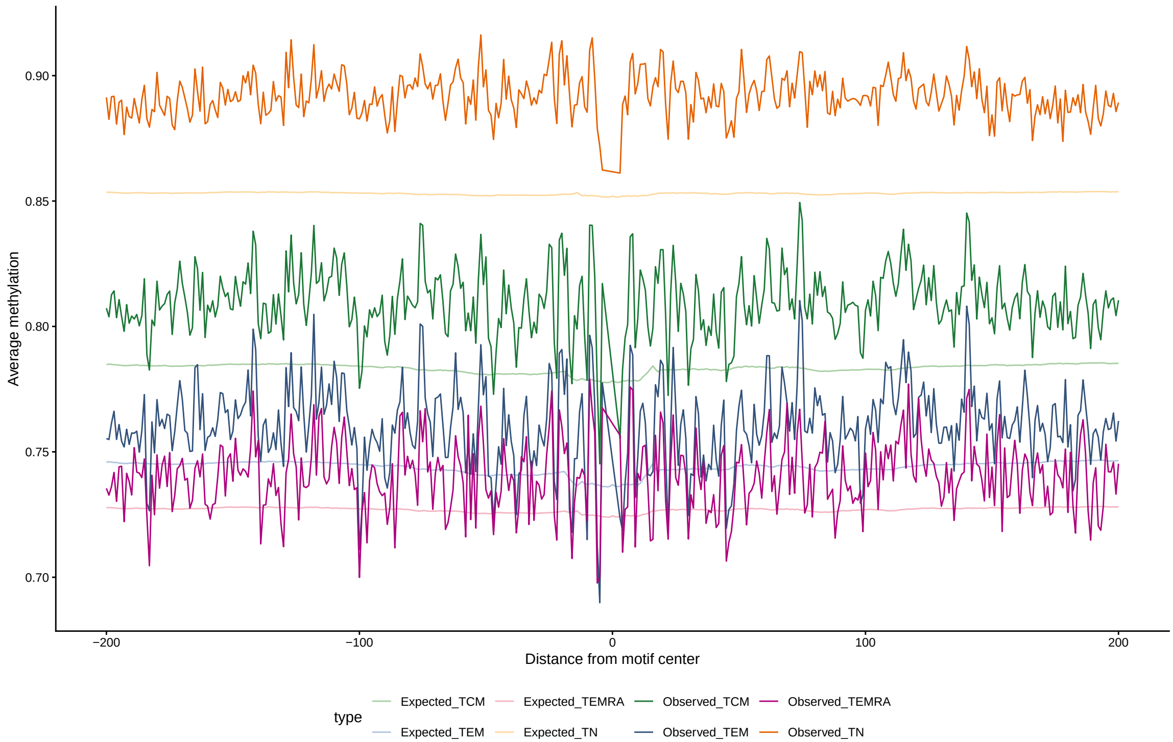
Expected vs observed footprints for RHOXF1
