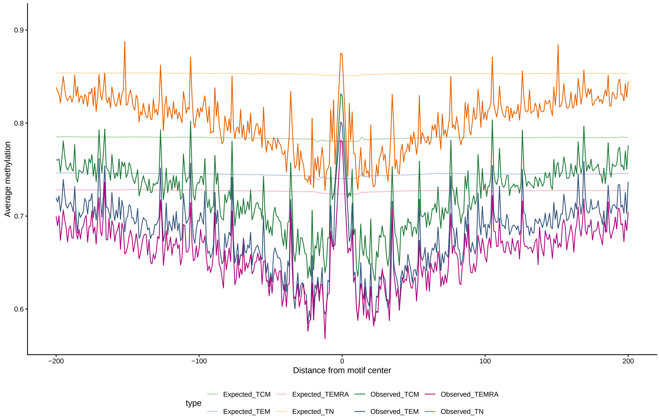
Expected vs observed footprints for RUNX2
