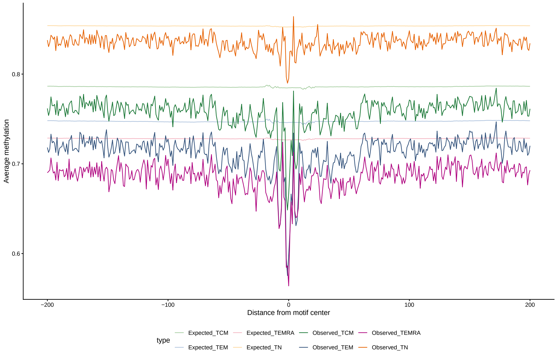
Expected vs observed footprints for RXRB
