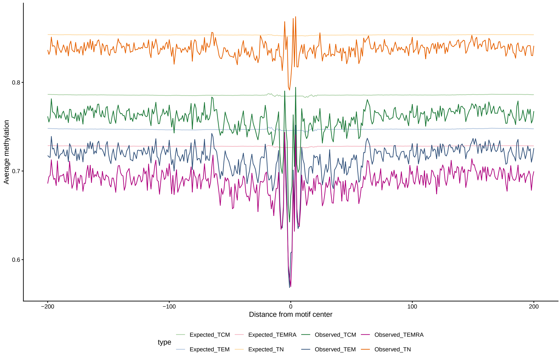
Expected vs observed footprints for RXRG
