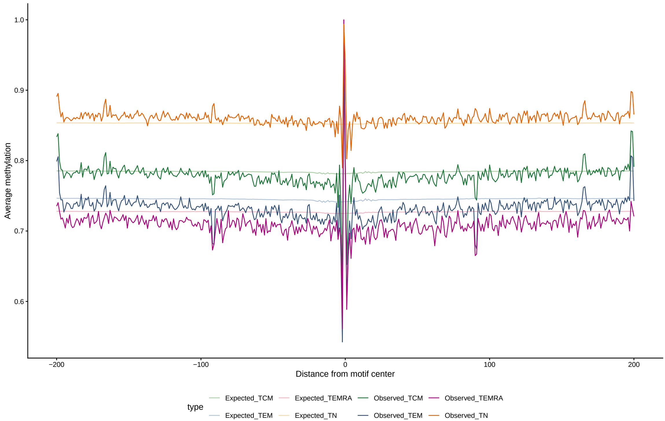
Expected vs observed footprints for SCRT1
