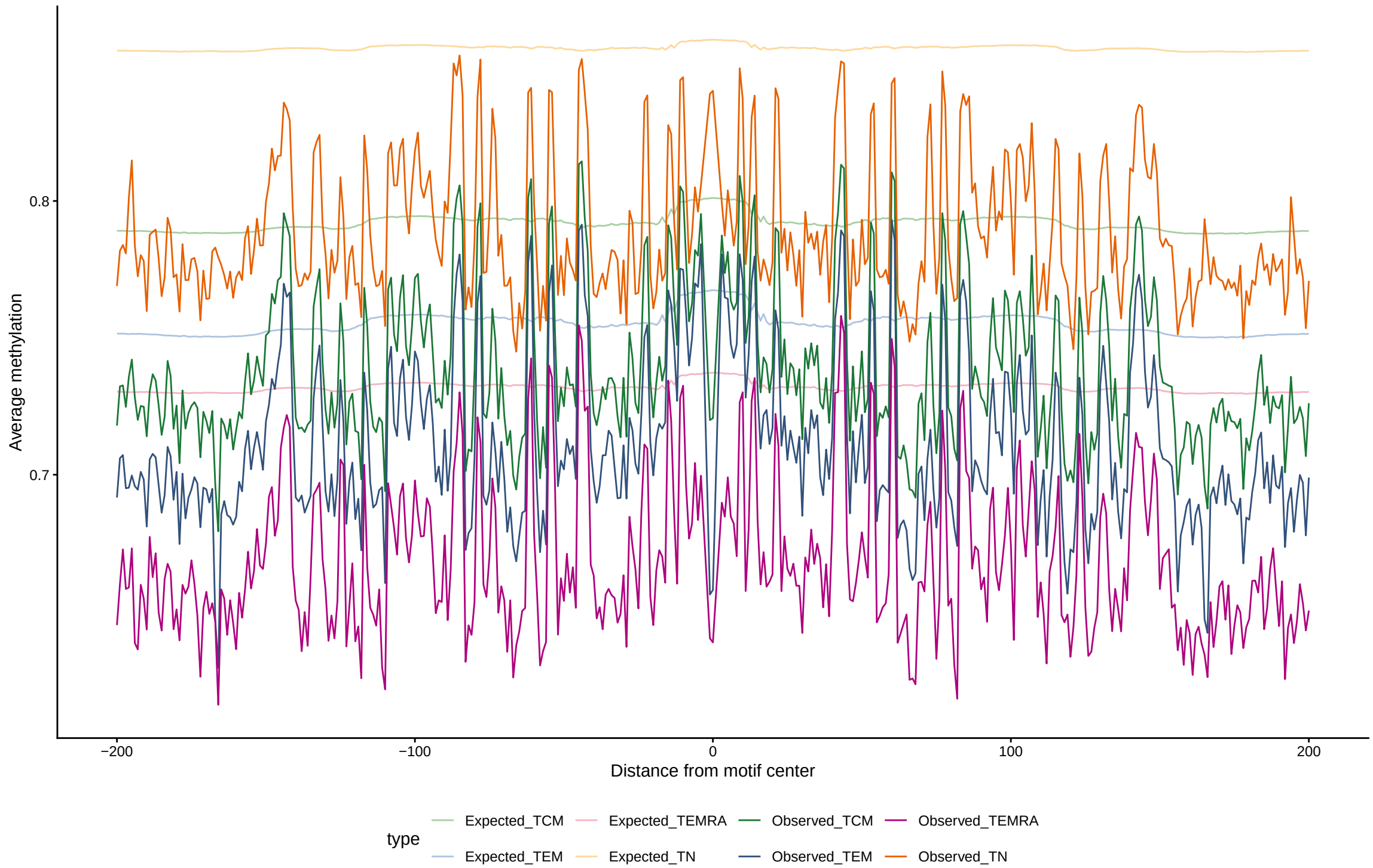
Expected vs observed footprints for SOHLH2
