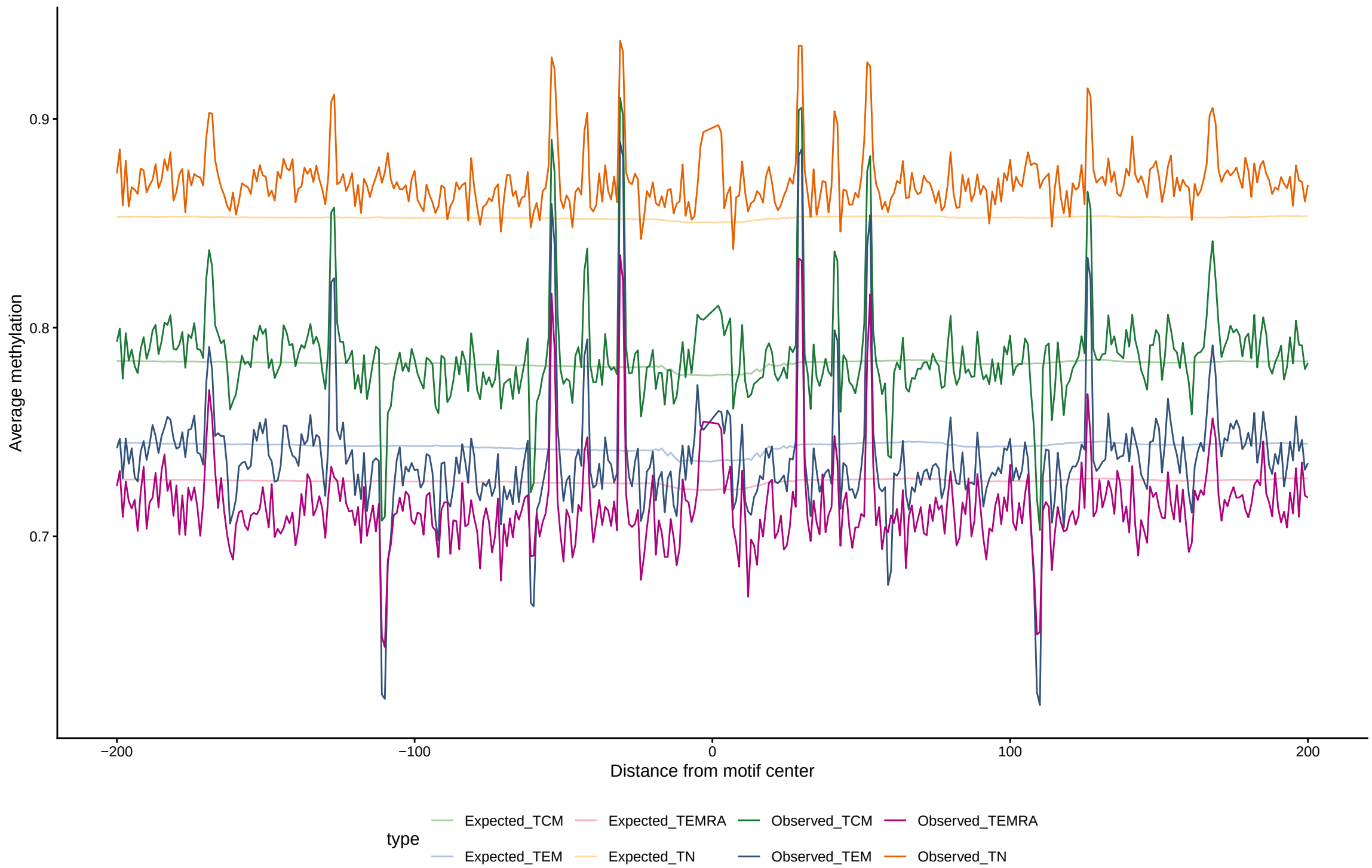
Expected vs observed footprints for SOX14
