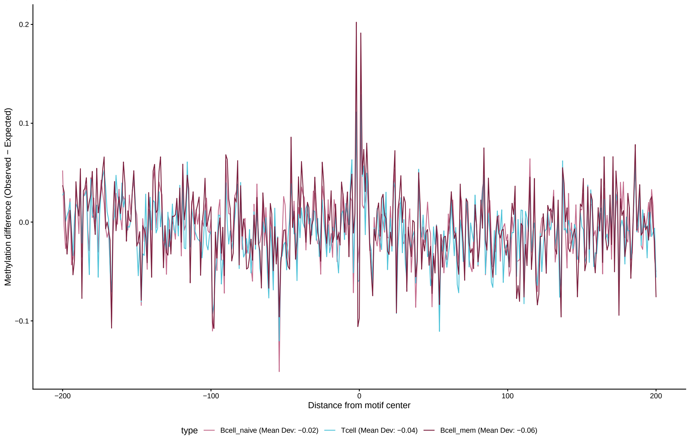
TF footprint difference for CREB3L4
