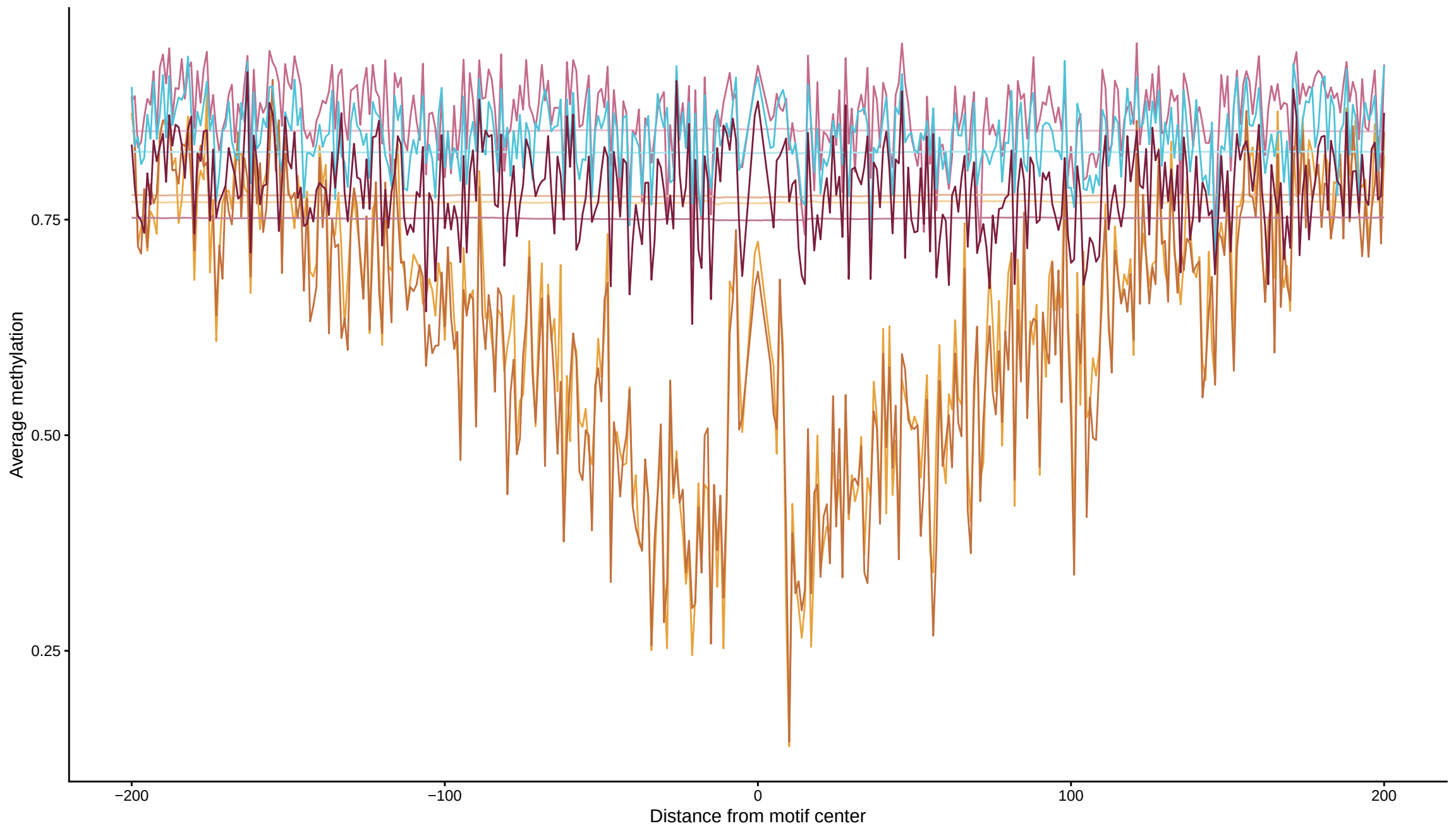
Expected vs observed footprints for CEBPB
