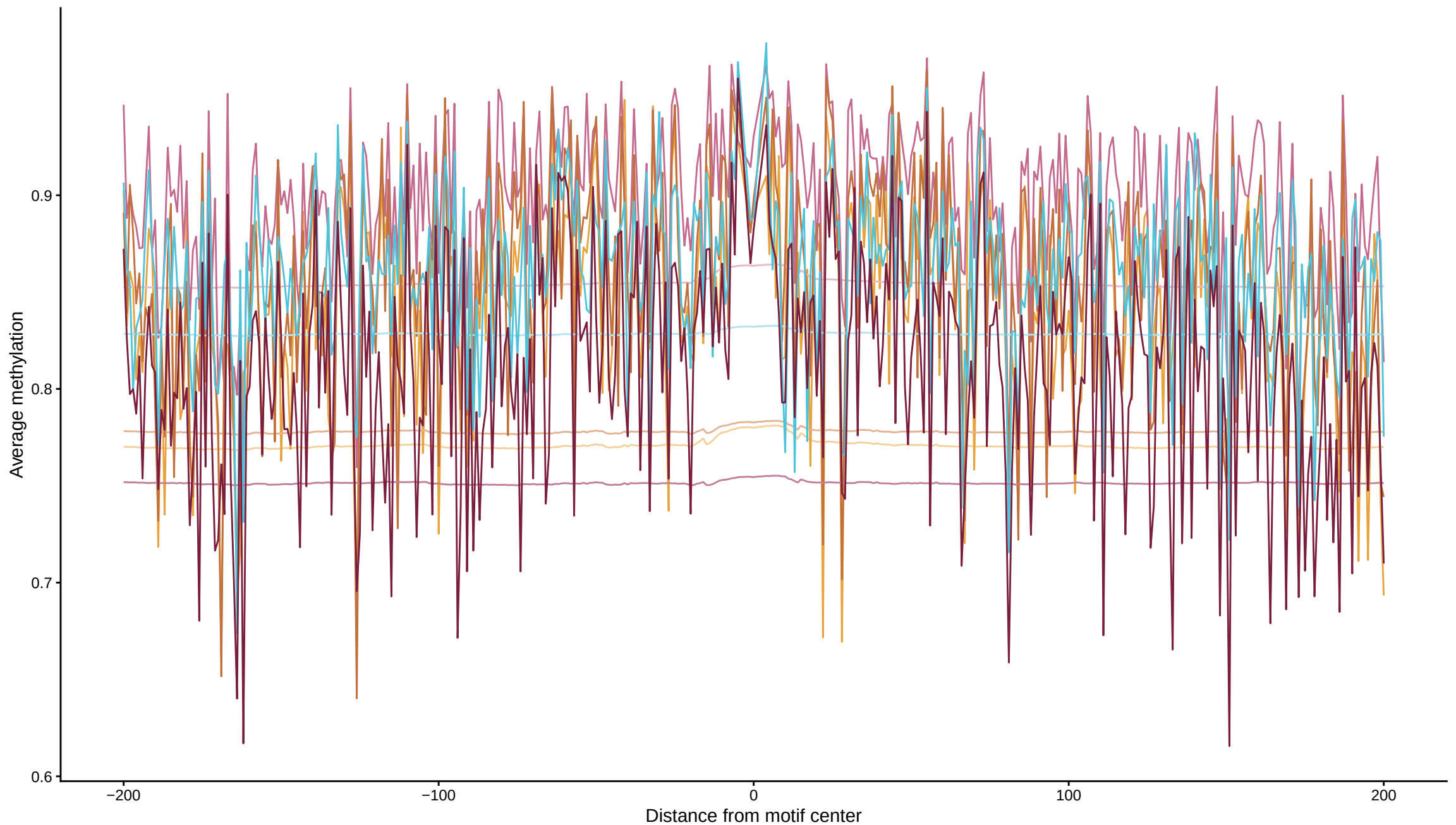
Expected vs observed footprints for CUX1
