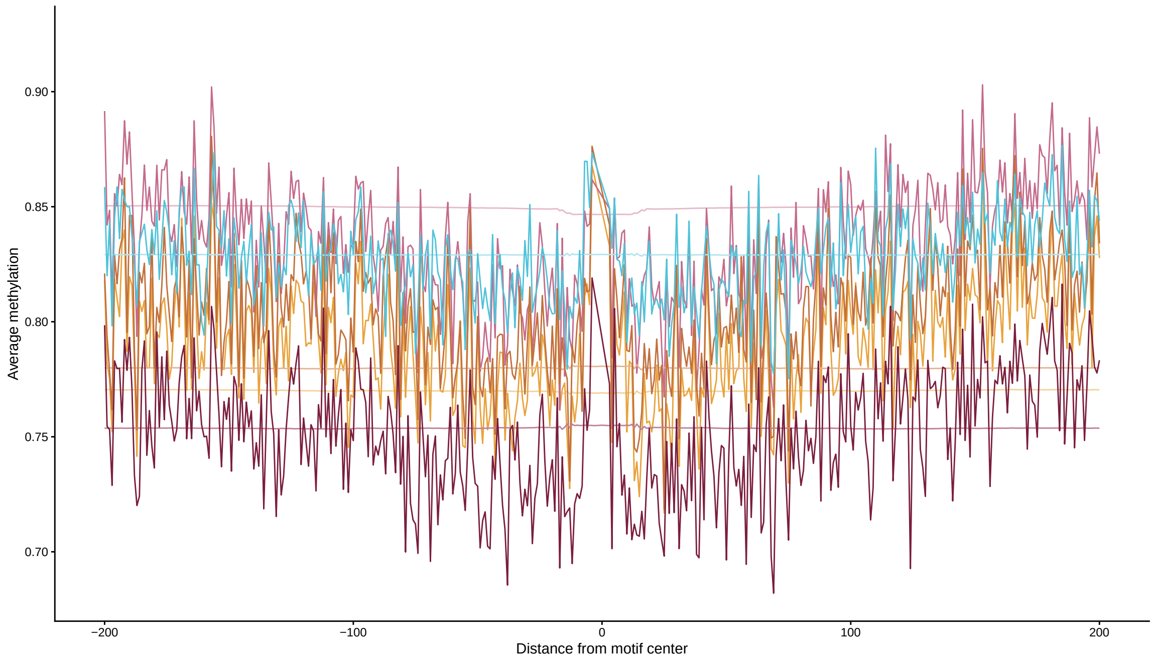
Expected vs observed footprints for MYF5
