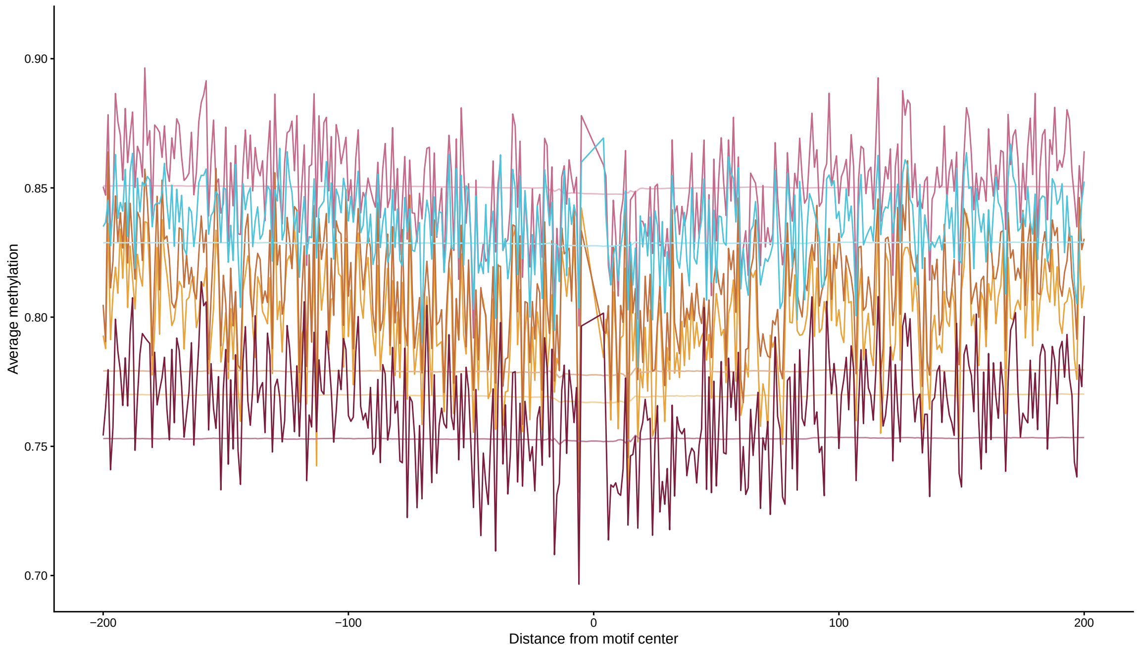
Expected vs observed footprints for NEUROD1
