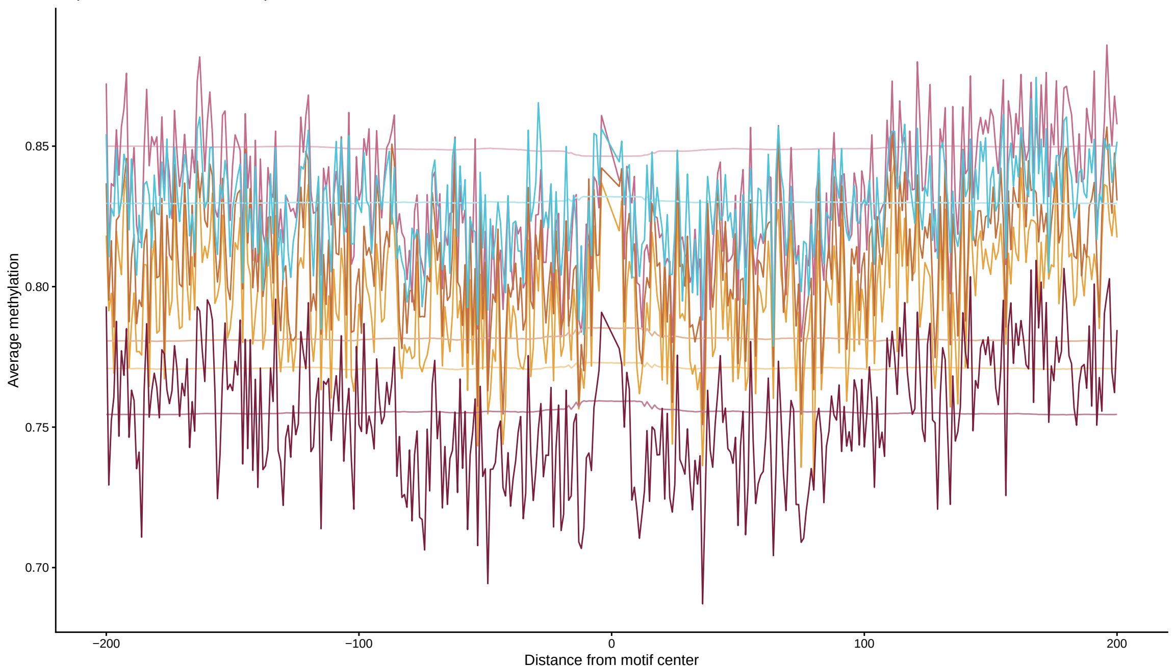
Expected vs observed footprints for NHLH1
