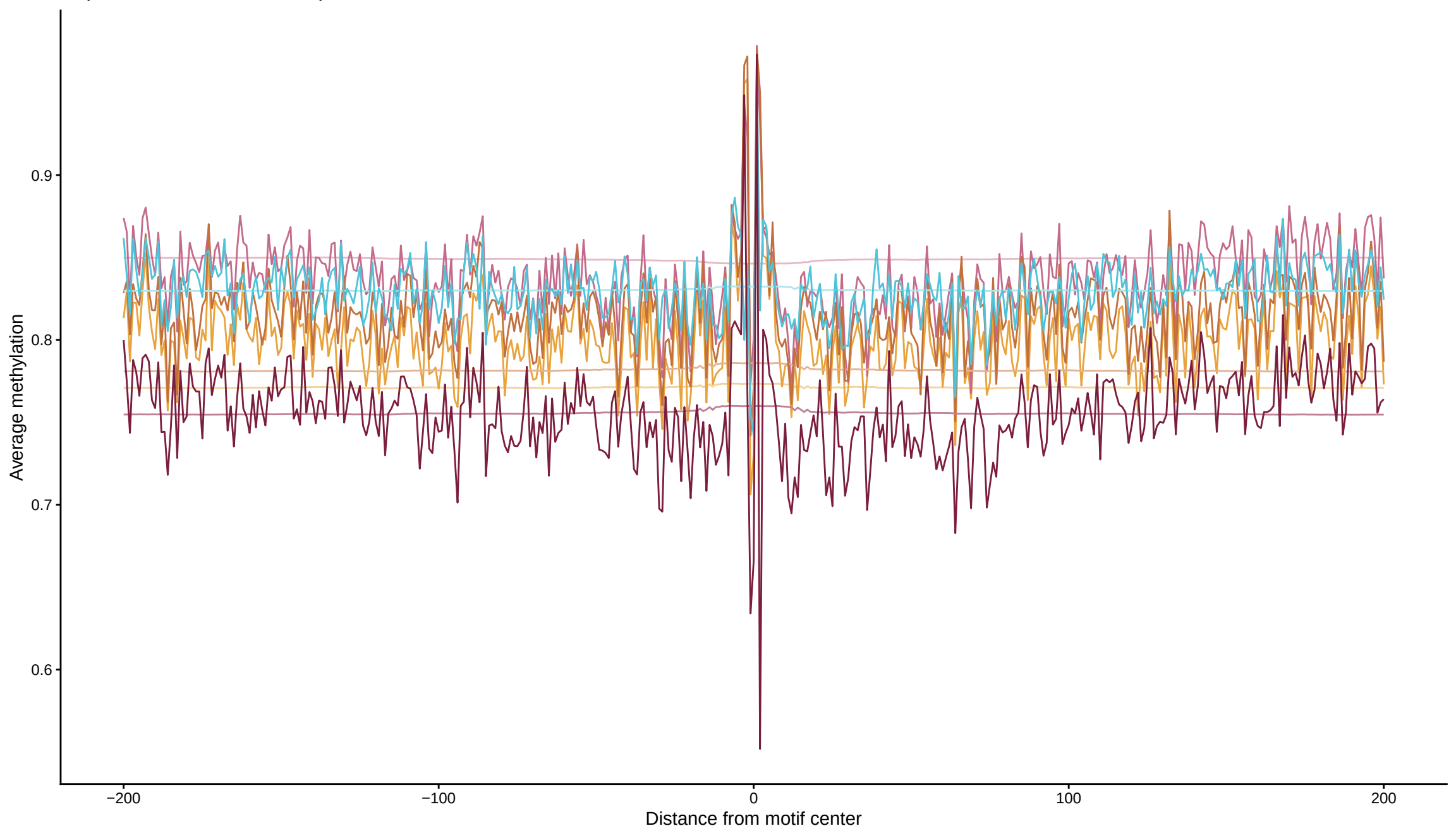
Expected vs observed footprints for NHLH2
