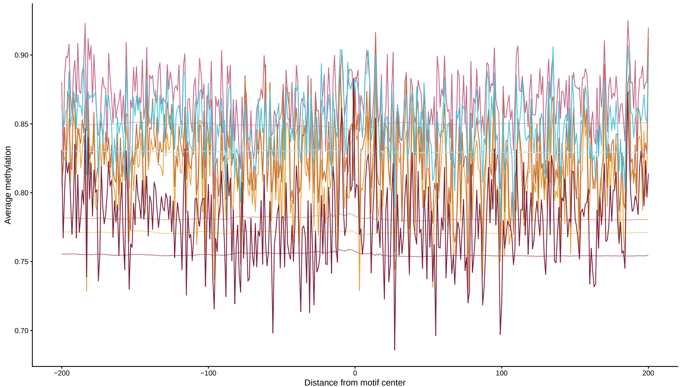
Expected vs observed footprints for PAX5
