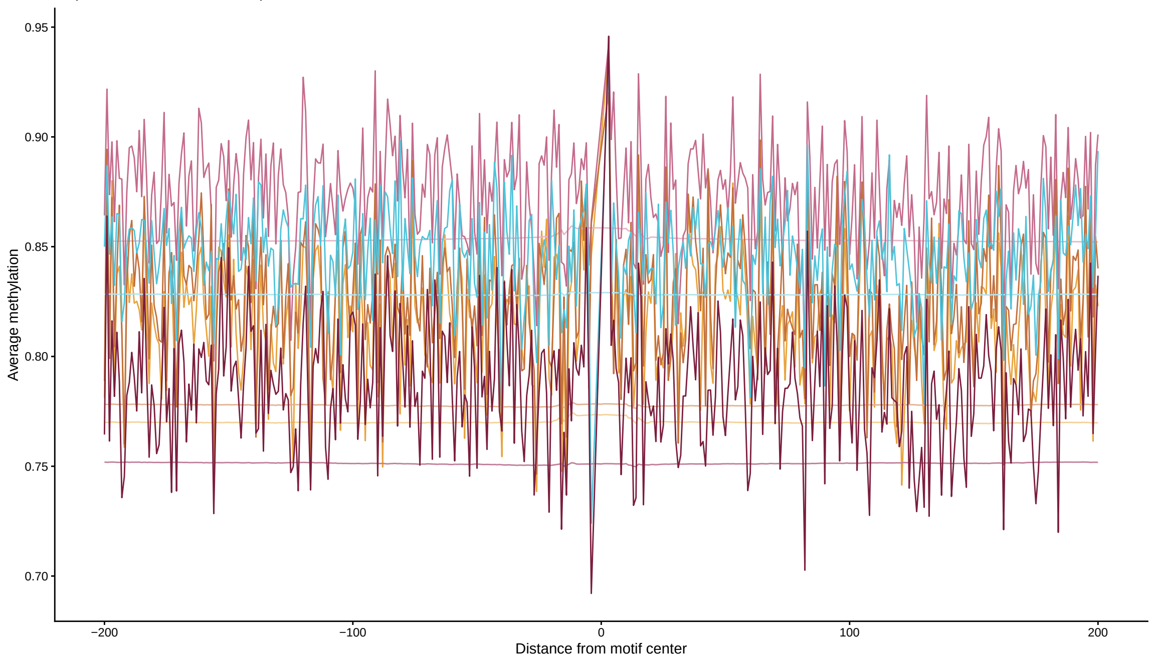
Expected vs observed footprints for SOX8
