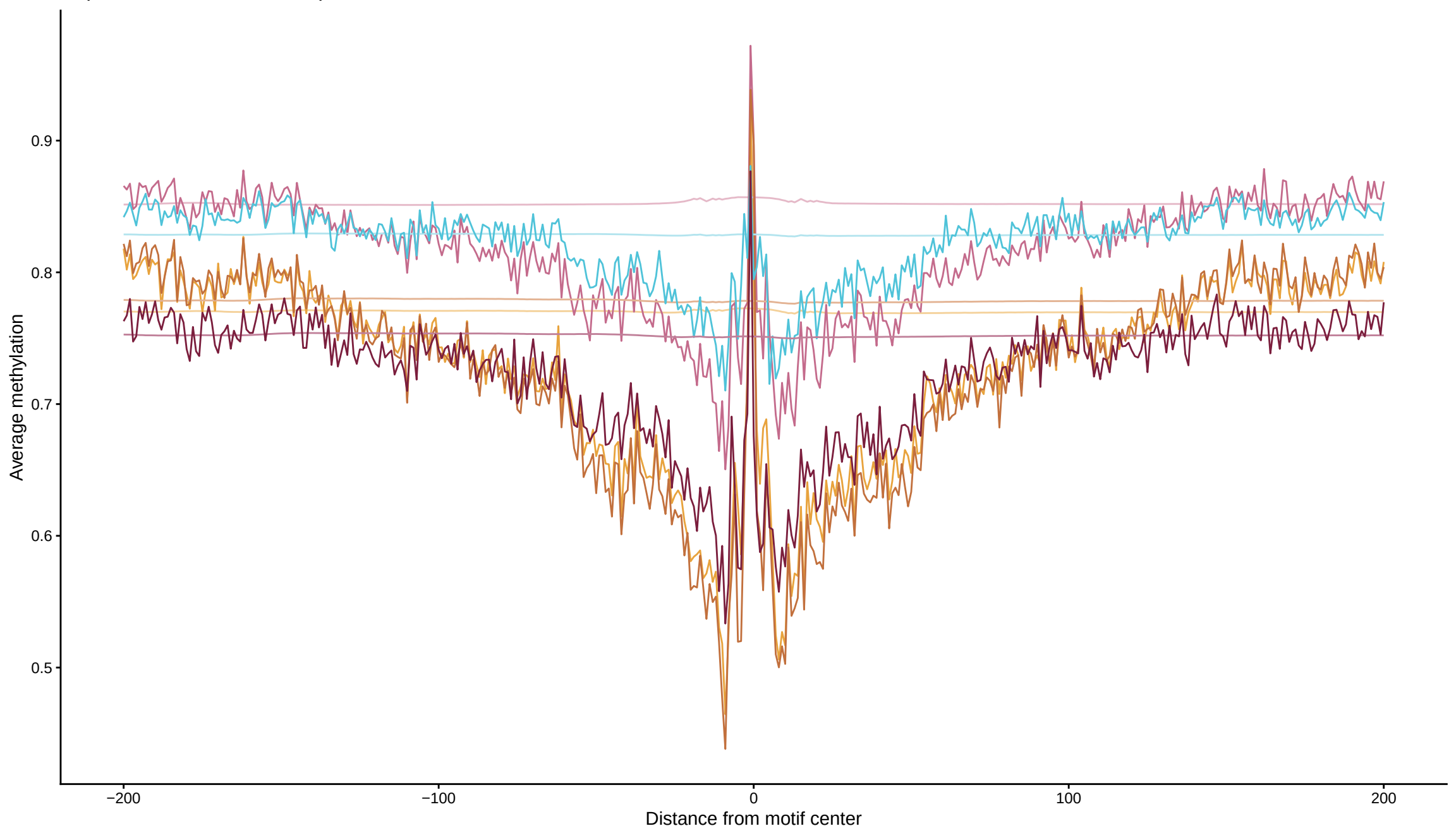
Expected vs observed footprints for SPI1
