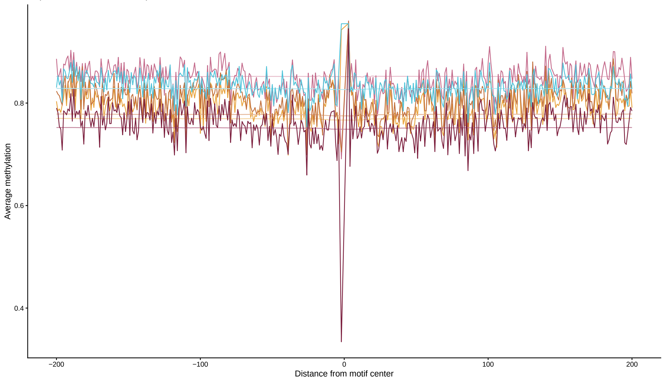
Expected vs observed footprints for TAL1::TCF3
