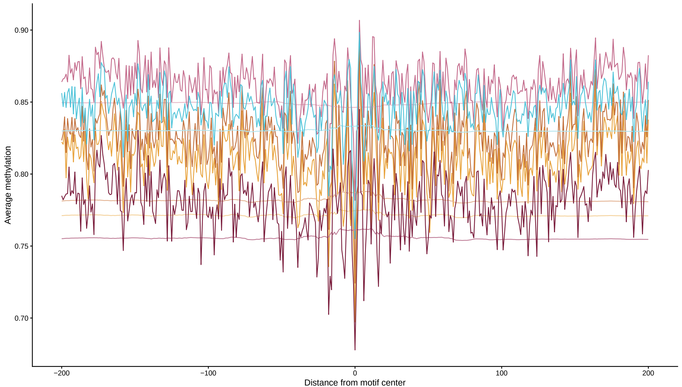
Expected vs observed footprints for TFAP2A
