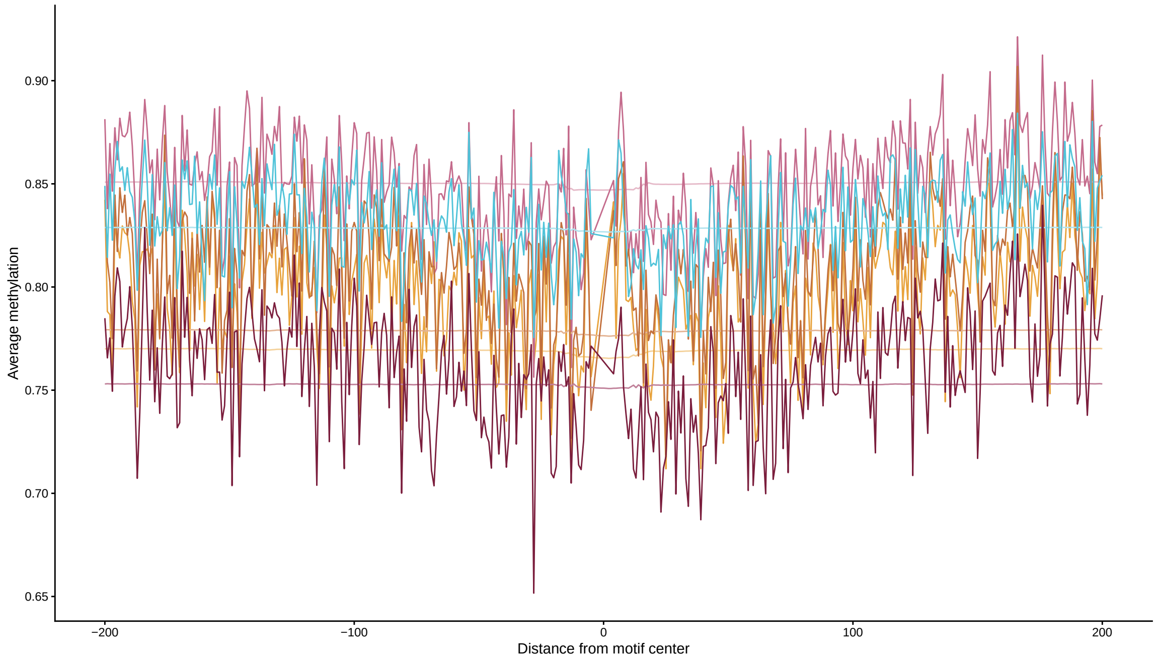
Expected vs observed footprints for TFAP4
