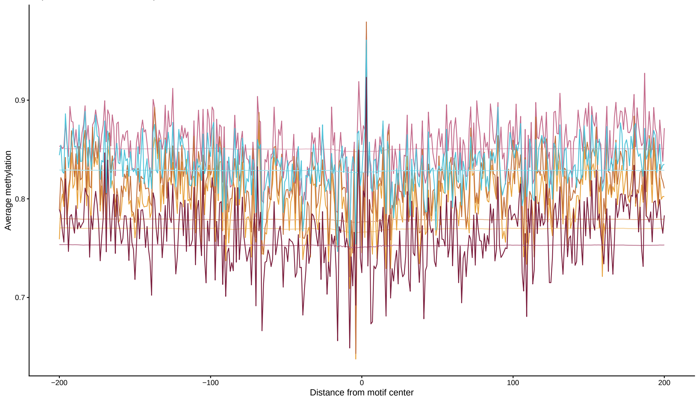
Expected vs observed footprints for TGIF1
