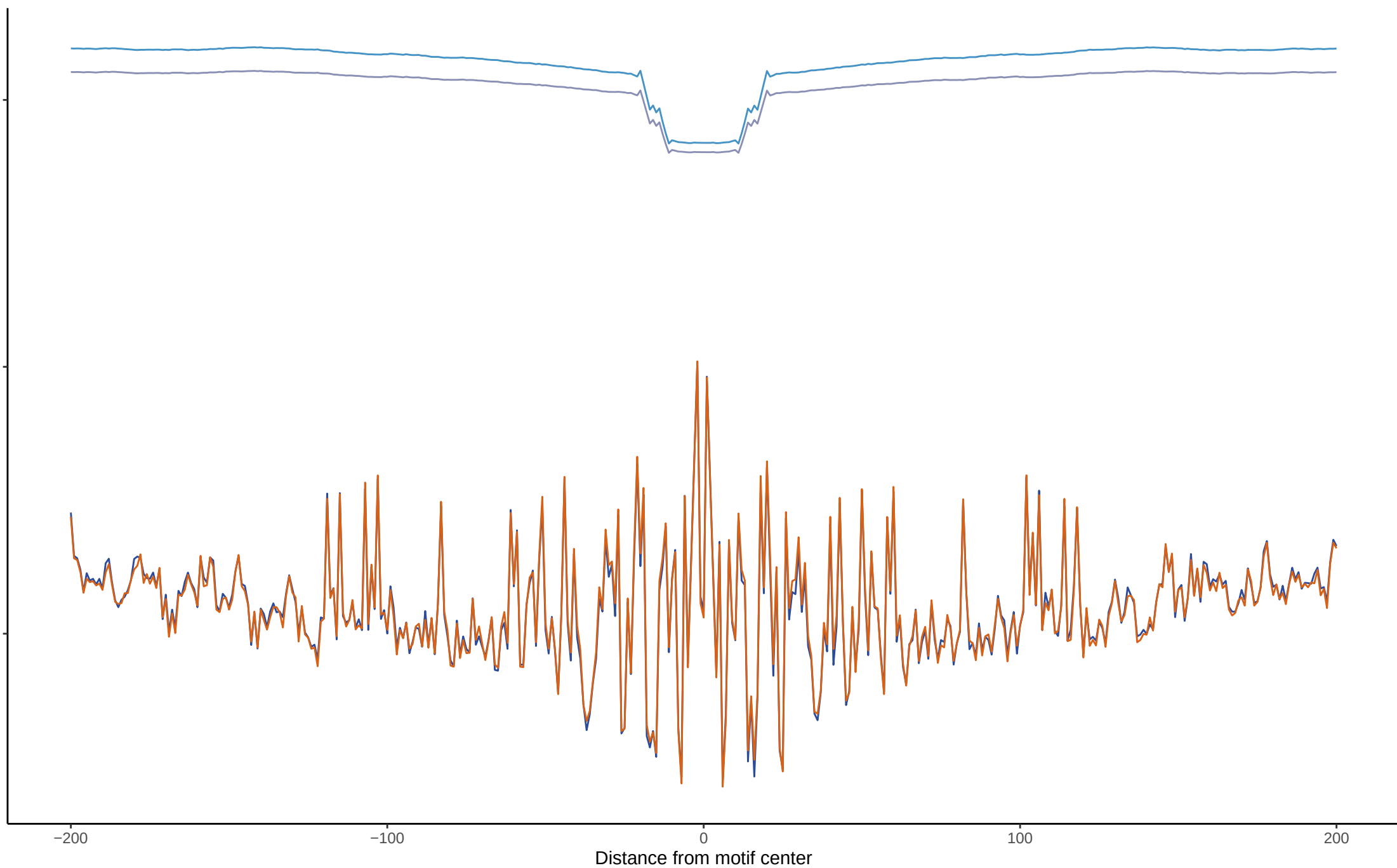
Expected vs observed footprints for TFAP2E
