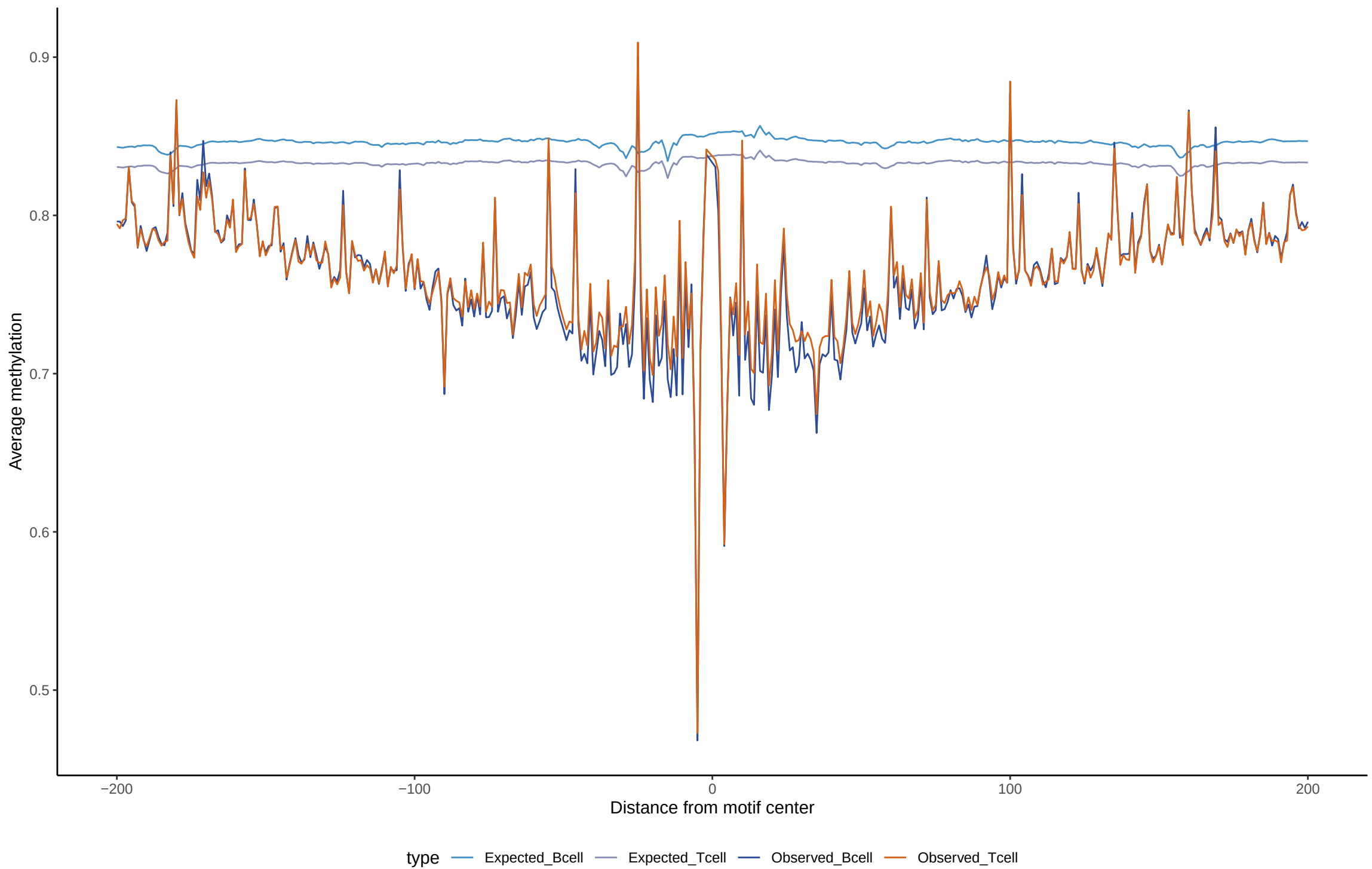
Expected vs observed footprints for ELF5
