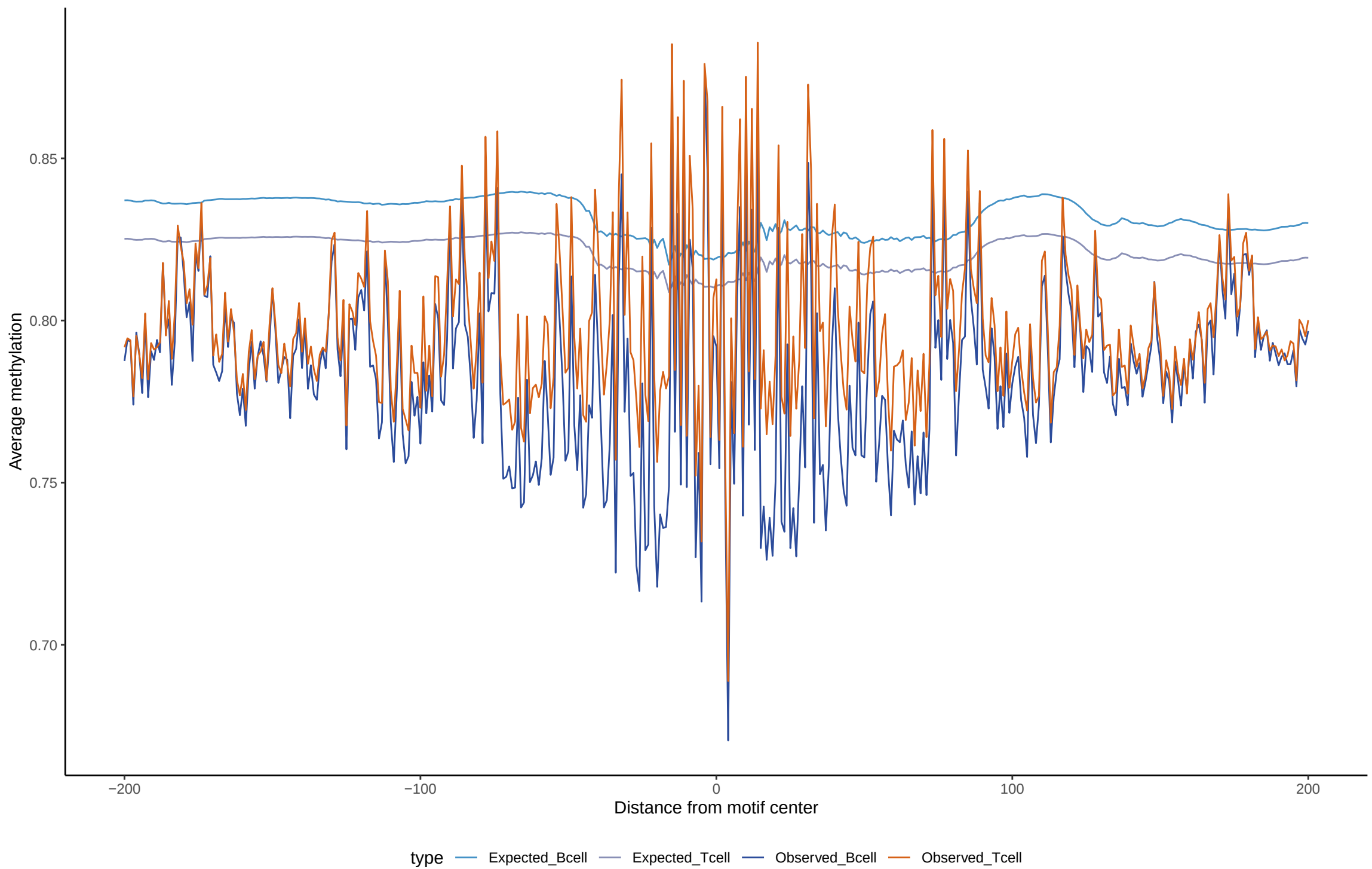
Expected vs observed footprints for PAX9
