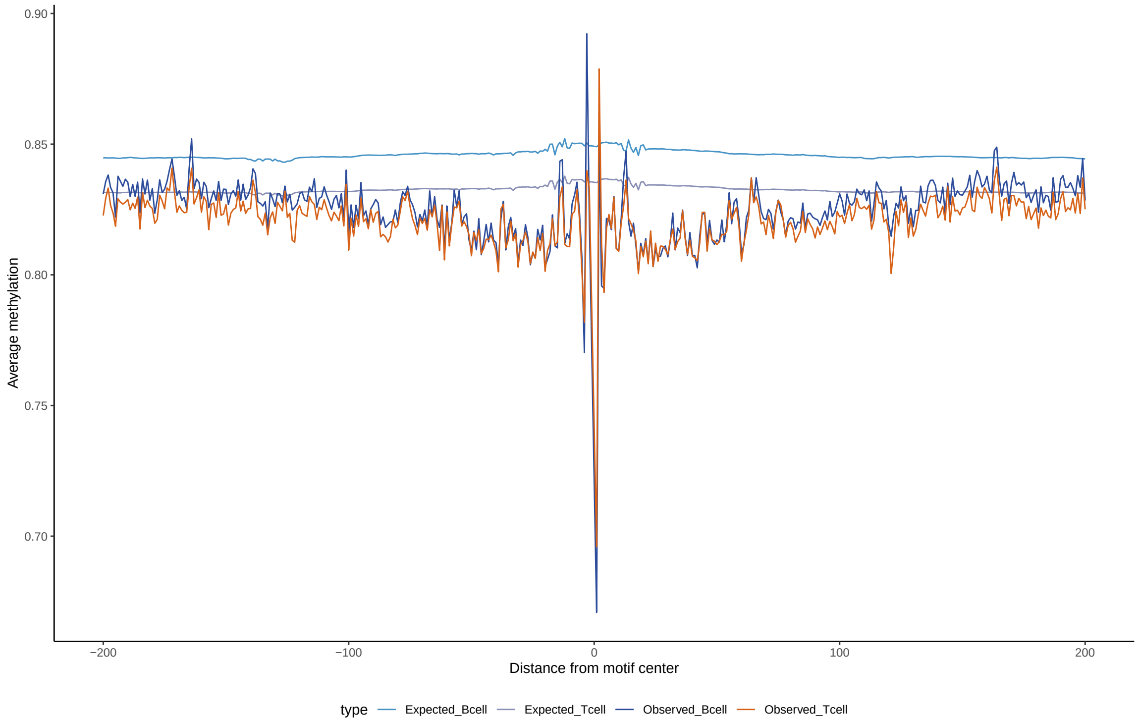
Expected vs observed footprints for TAL1::TCF3
