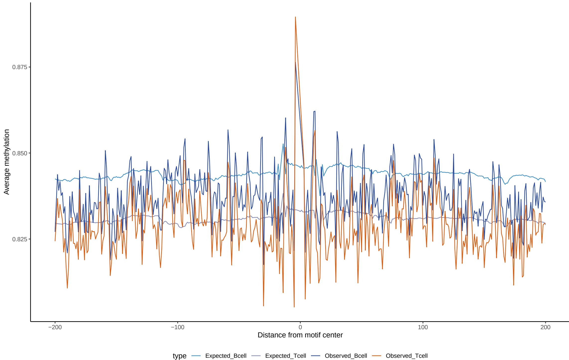
Expected vs observed footprints for TEAD3
