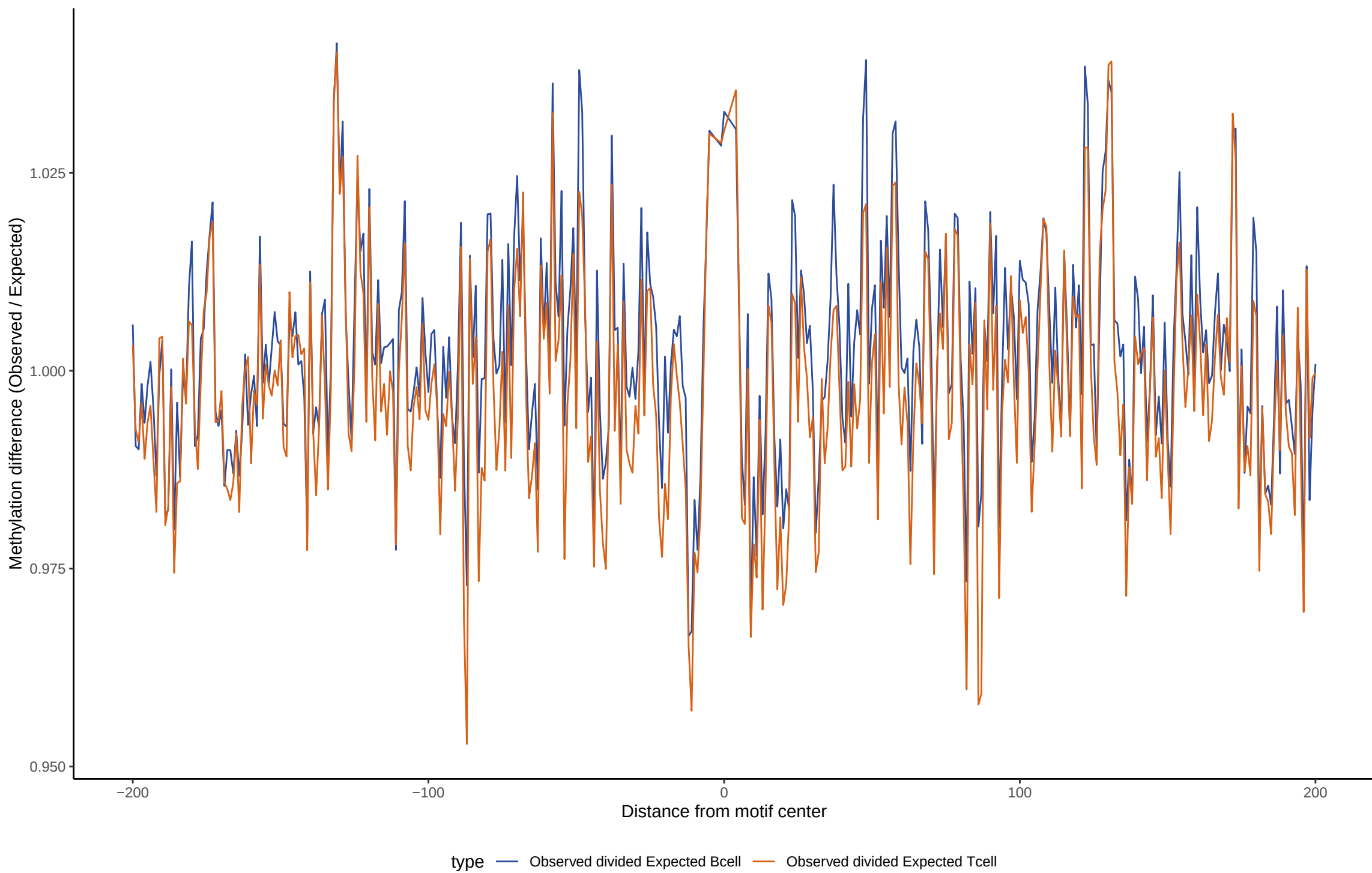
TF footprint difference for CUX1
