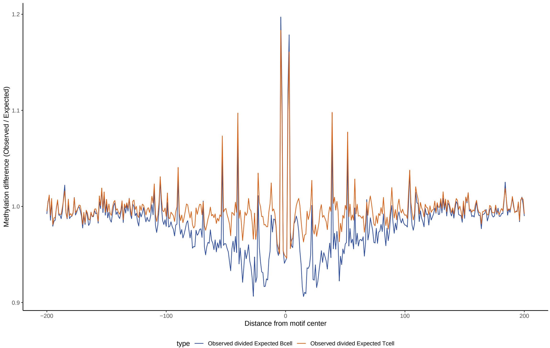
TF footprint difference for EBF3
