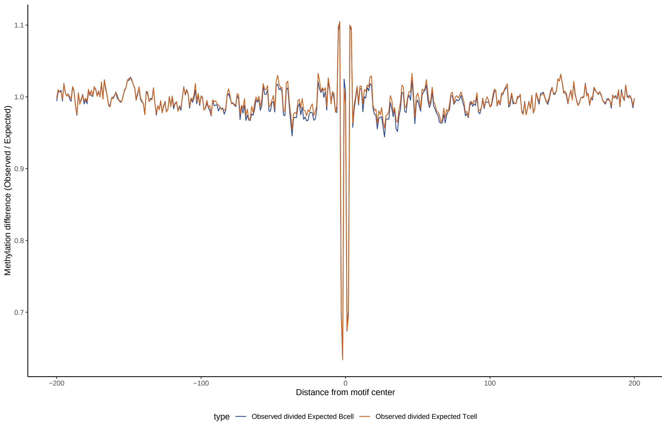
TF footprint difference for NHLH2
